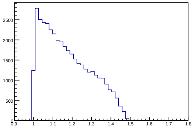
ElectronPt
