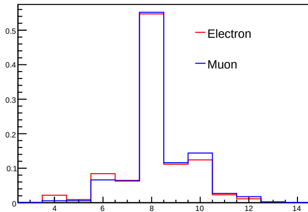
PixelSCTHits
