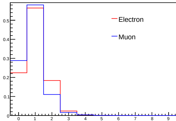
CountMuon
