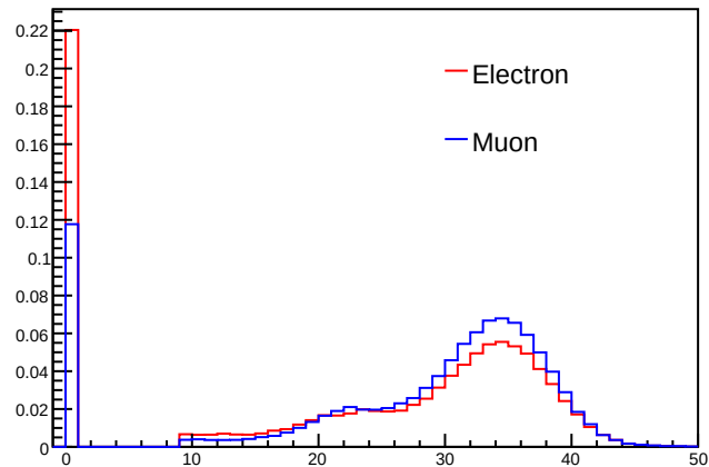
PixelTRTHits
