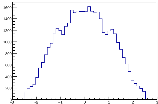
ElectronEta
