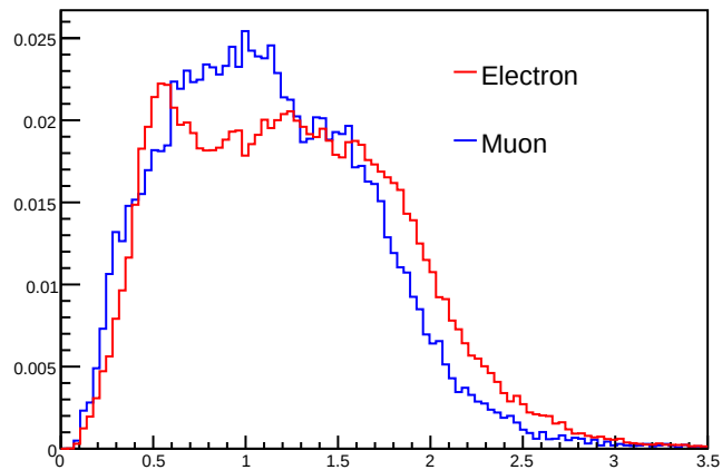
Transversal momentum
