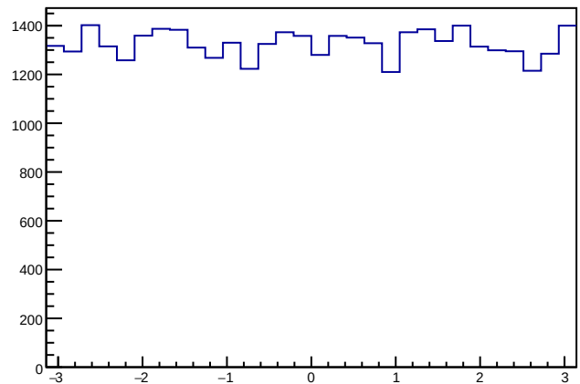
ElectronPhi
