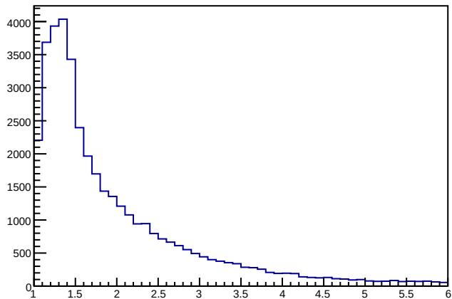
ElectronEnergy
