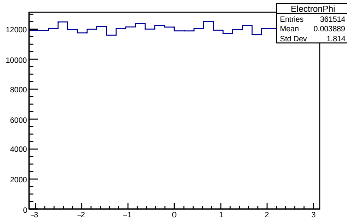
ElectronPhi
