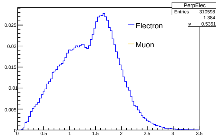
Transversal momentum
