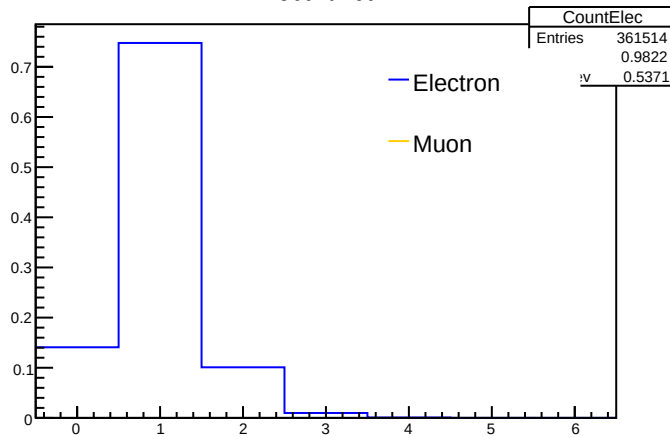
CountElec
