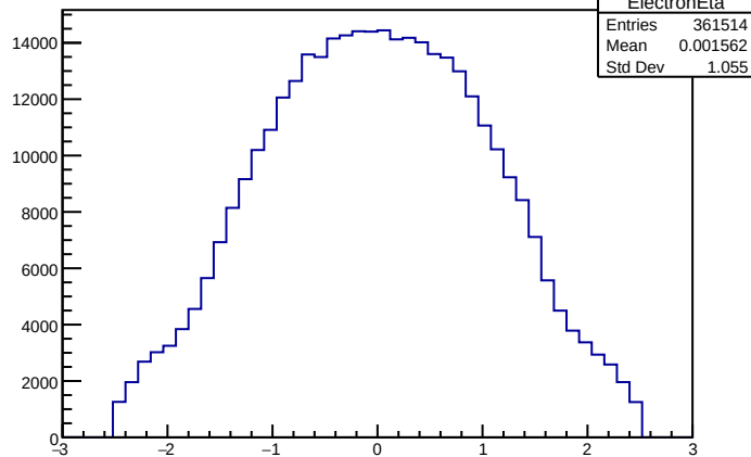
ElectronEta
