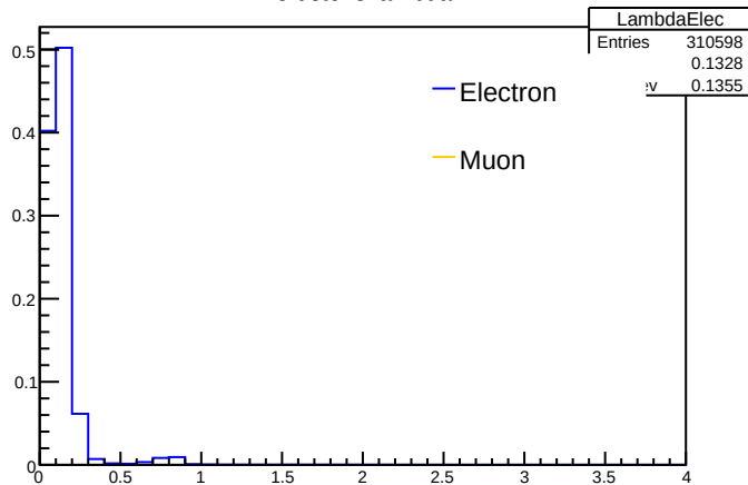
Cluster's lambda
