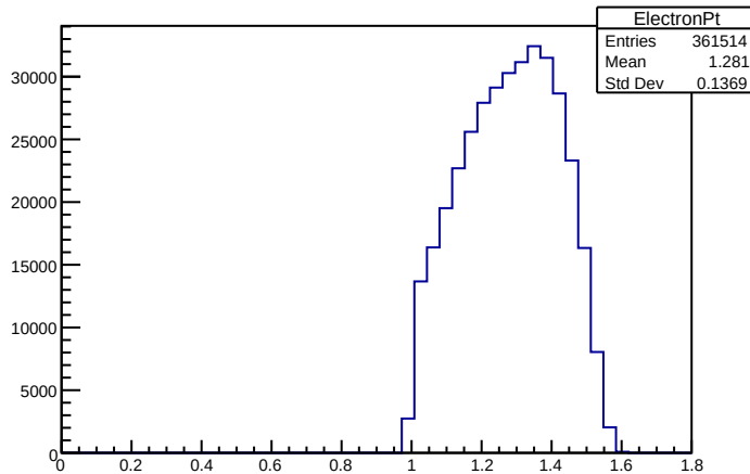
ElectronPt
