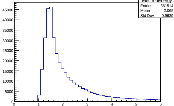
ElectronEnergy
