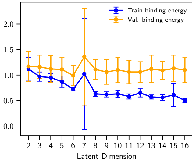
Binding Energy MAE (kJ/mol)
