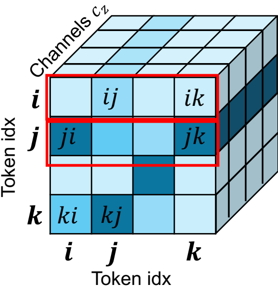
Pair representation z
