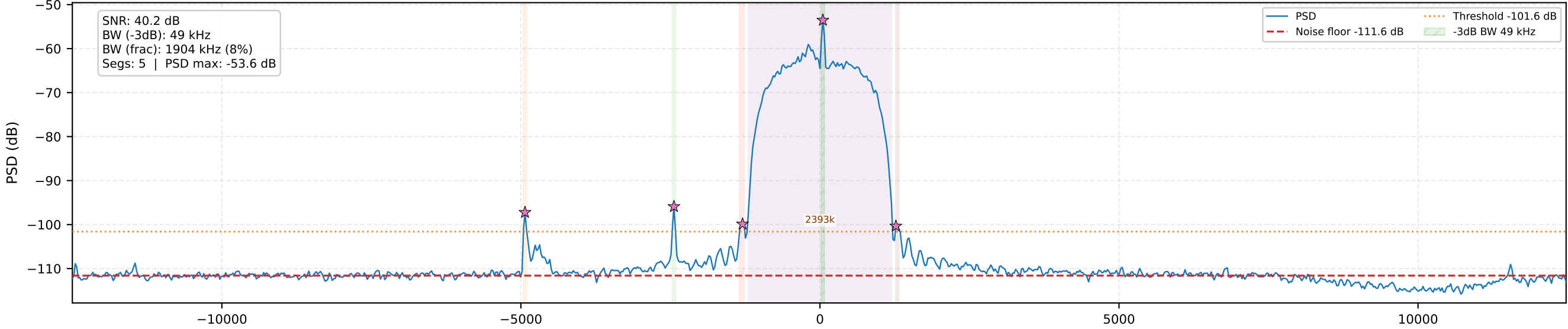
EMISignal1_demod_train_0000 — EMISignal1 | demod | 1.64 ms, 40,960 samples
