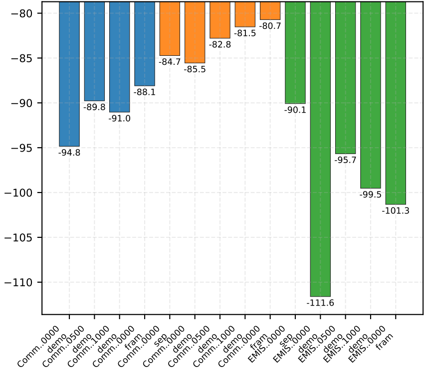
Noise Floor (MAD, dB)
