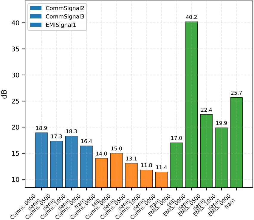
SNR (PSD-based, dB)
