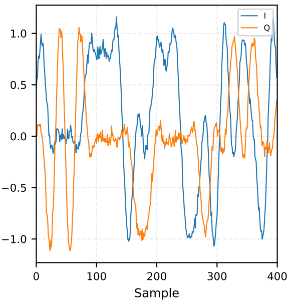
CommSignal2_demod_train_0000 — I/Q vs Time (raw)
