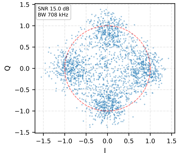
Constellation (normalized)
