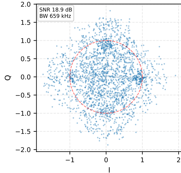
Constellation (normalized)
