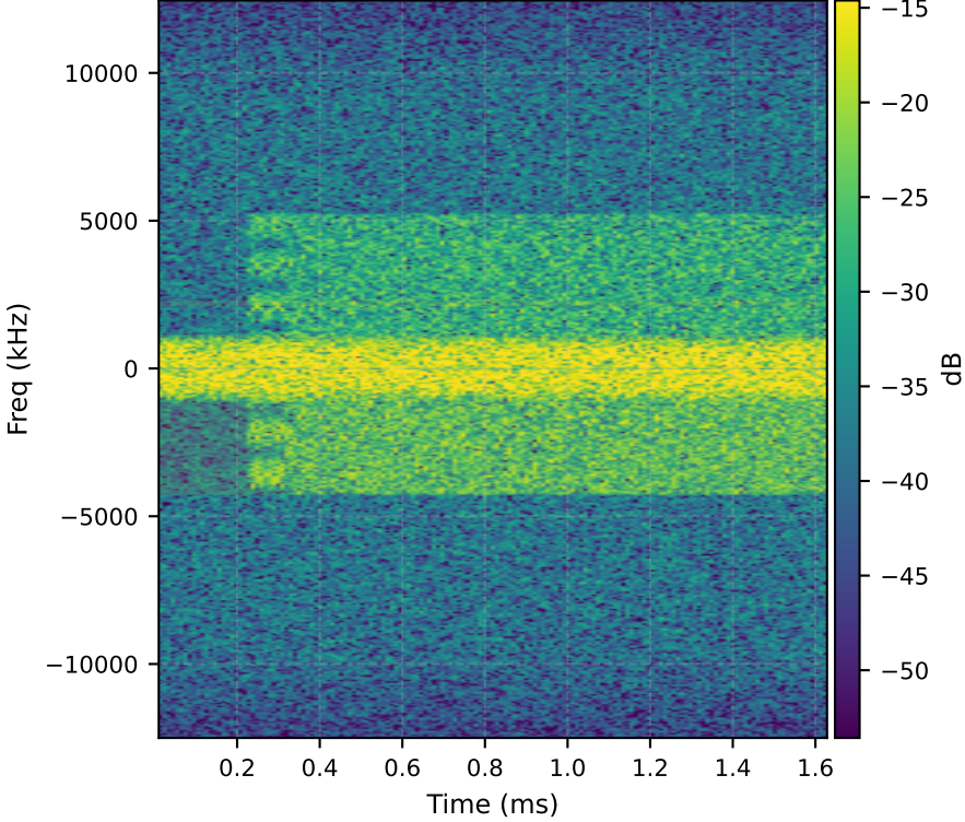
Spectrogram
