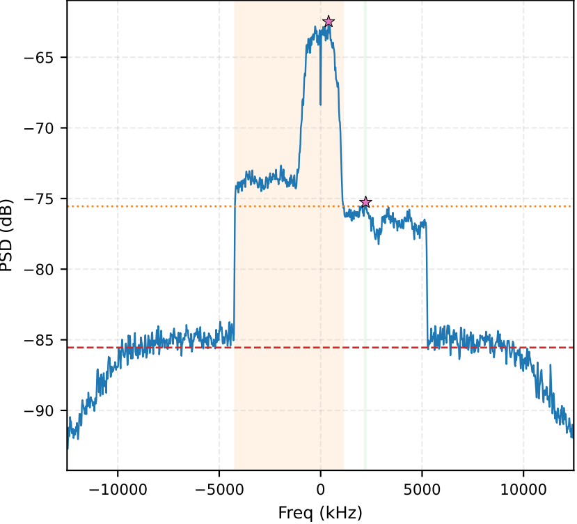
PSD — 2 segments
