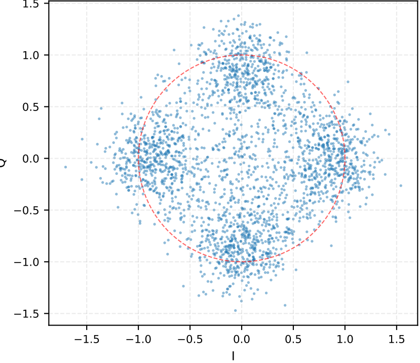
Constellation (normalized, 2500 pts)
