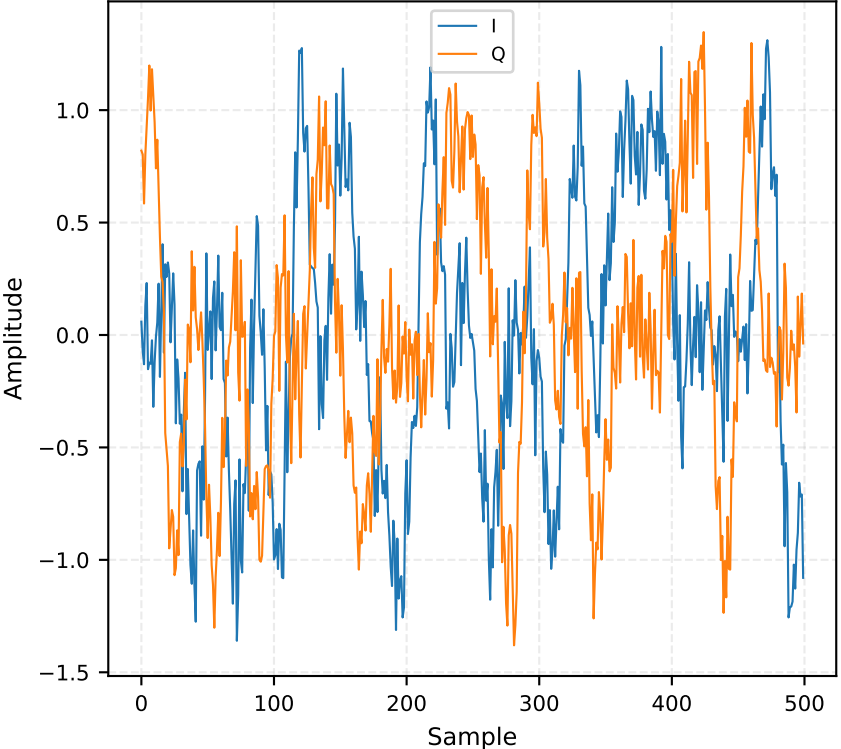
I/Q vs Time — first 500 samples (raw)
