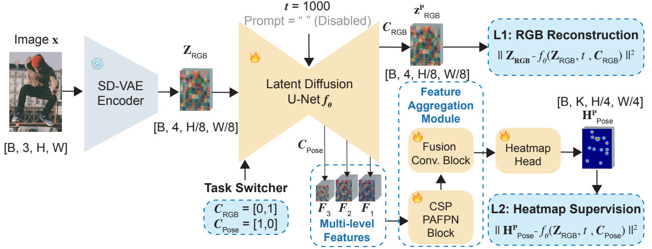
Figure 3: Training pipeline of SDPose. The input image x is encoded by a pre-trained SD-VAE into Z_{\text{RGB}} . A shared latent diffusion U-Net f_{\theta} is conditioned by a task/class embedding C (text prompt disabled). With C_{\text{RGB}} , the model reconstructs Z_{\text{RGB}} via an \ell_2 latent reconstruction loss. With C_{\text{Pose}} , we extract selected multi-level U-Net features, perform feature aggregation, and predict keypoint heatmaps supervised by a heatmap MSE loss.
