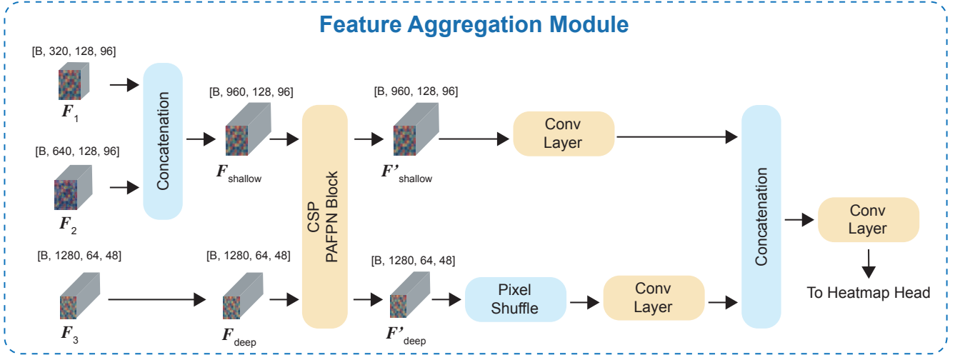
Figure 9: Hierarchical features are fused through a CSP PAFPN block. Deep features are upsampled via PixelShuffle to align with shallow features for final heatmap prediction.
