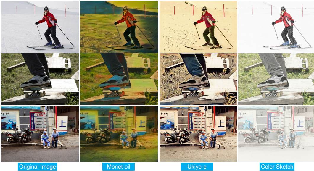
Figure 8: Visual illustration of the style-transferred subsets in the COCO-OOD benchmark. We create an OOD split of the COCO validation set by stylizing natural images into three distinct artistic domains: Monet (via StyTR2), Ukiyo-e (via CycleGAN), and Color-sketch (via Nano Banana), enabling comprehensive evaluation under diverse style shifts.
