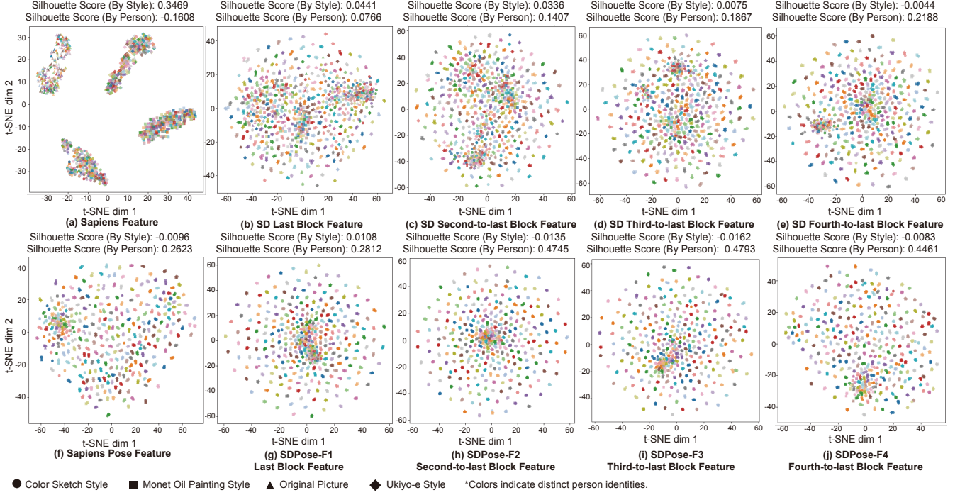
Figure 2: t-SNE visualization of features from Sapiens ViT, Stable Diffusion U-Net blocks, Sapiens Pose, and SDPose across four visual domains. Each point corresponds to an image sample; colors represent person instances and marker shapes denote artistic styles.
