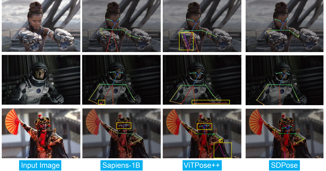
Figure 4: Qualitative results on real-world photographs. The yellow boxes highlight regions where baselines fail to predict accurate poses.
