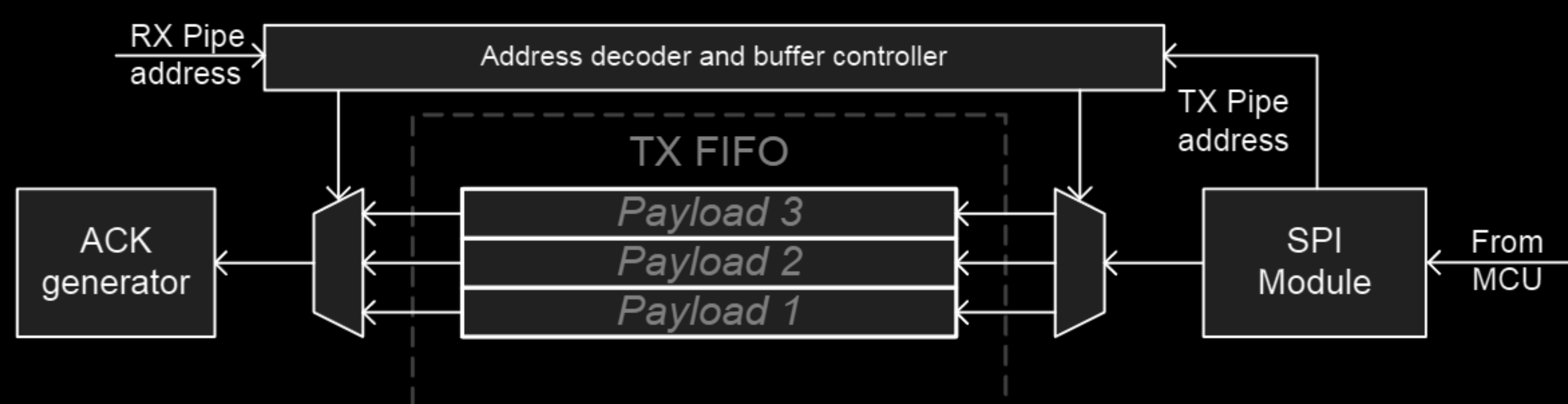
Figure 9. TX FIFO (PRX) with pending payloads
