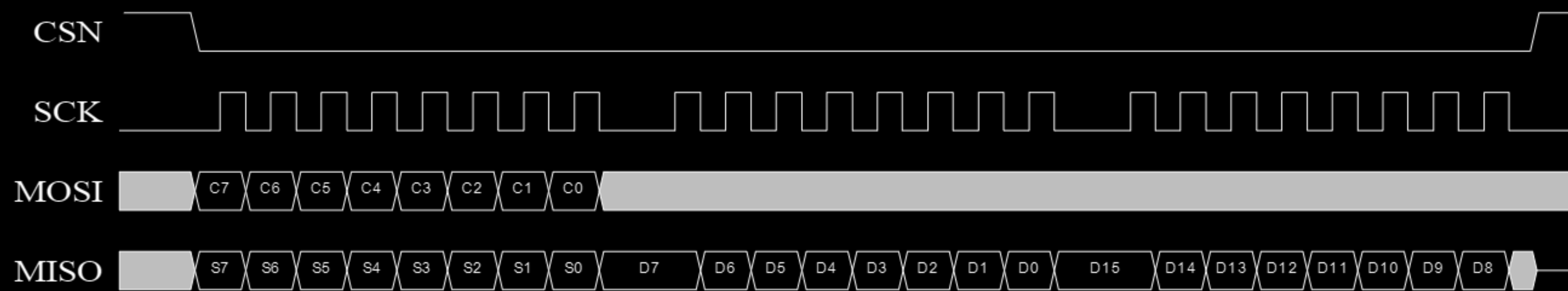
Figure 26. SPI read operation
