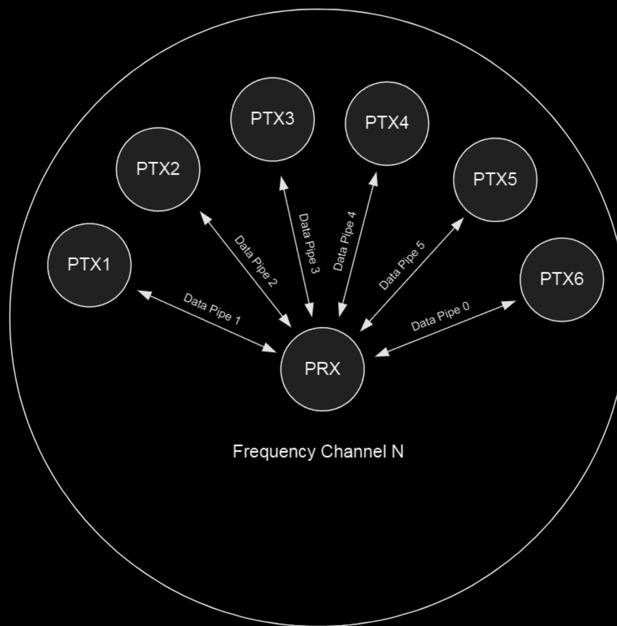
Figure 12. PRX using MultiCeiver™
