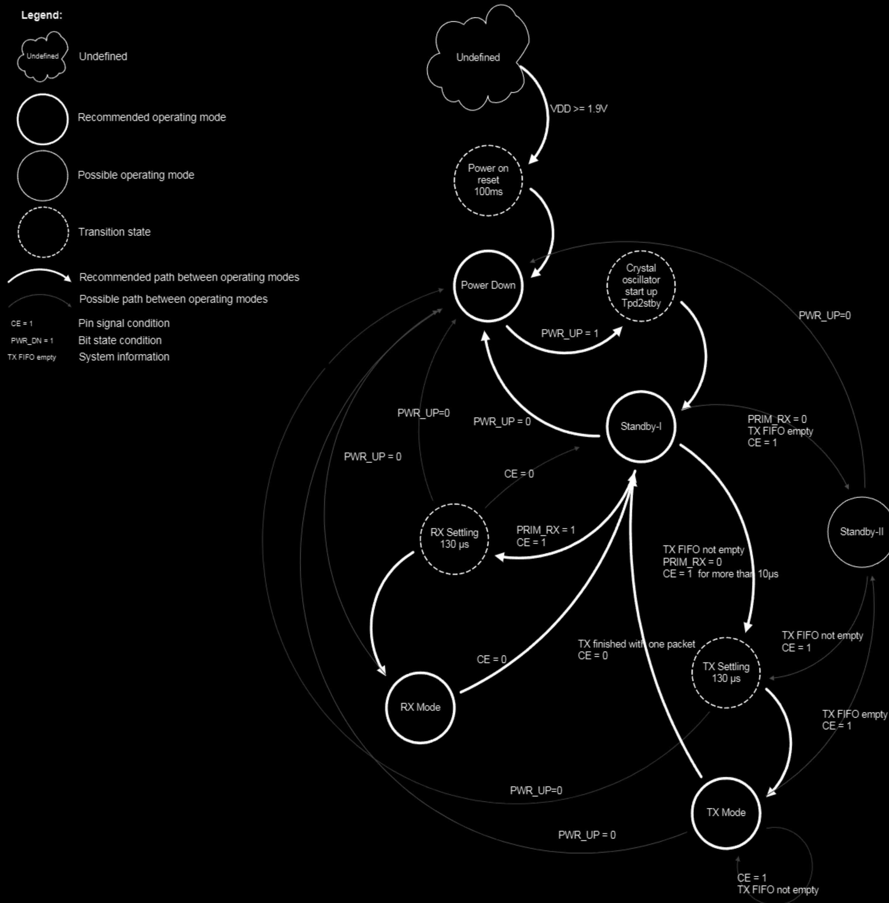
Figure 4. Radio control state diagram
