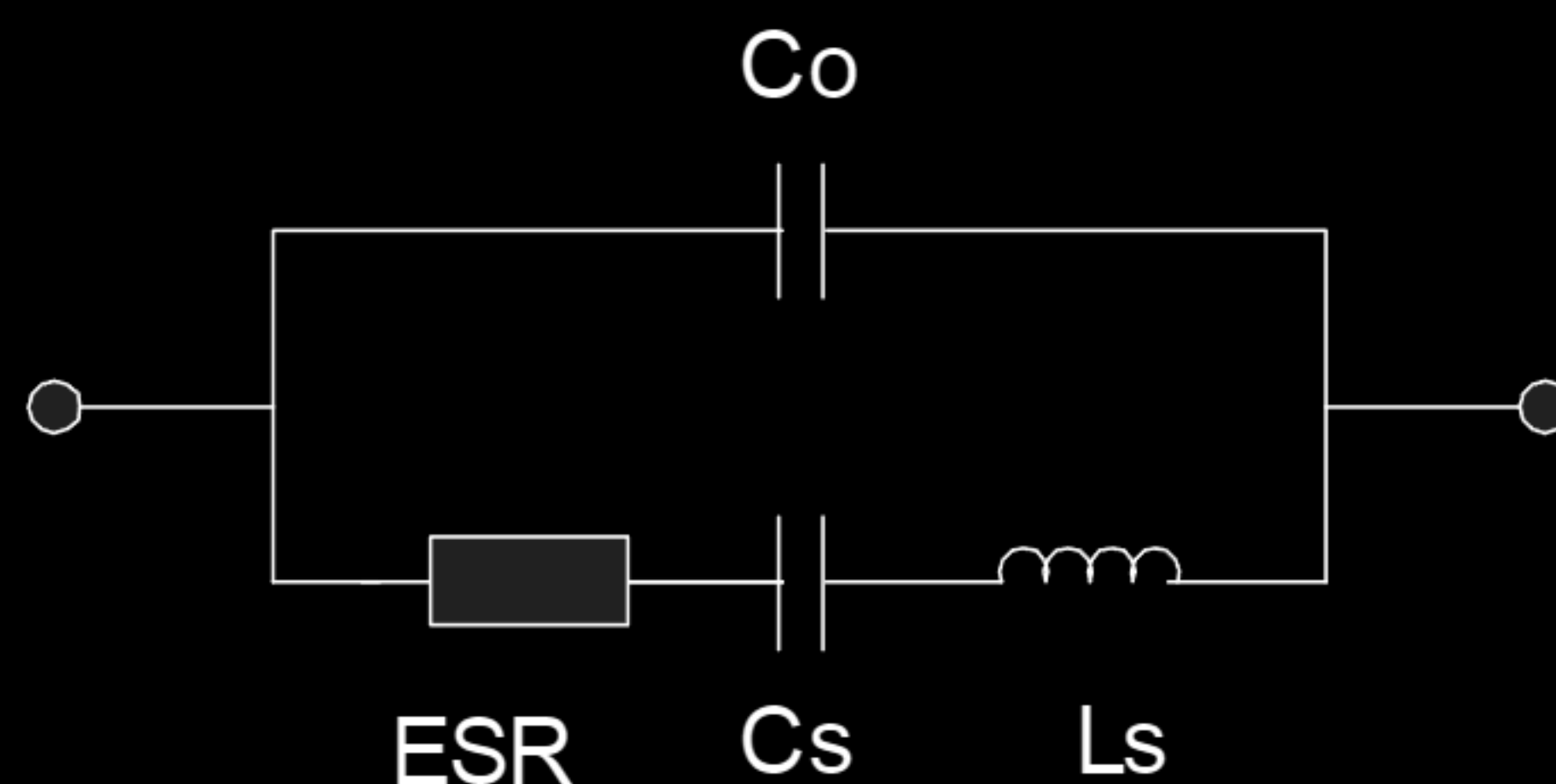
Figure 3. Equivalent crystal components
