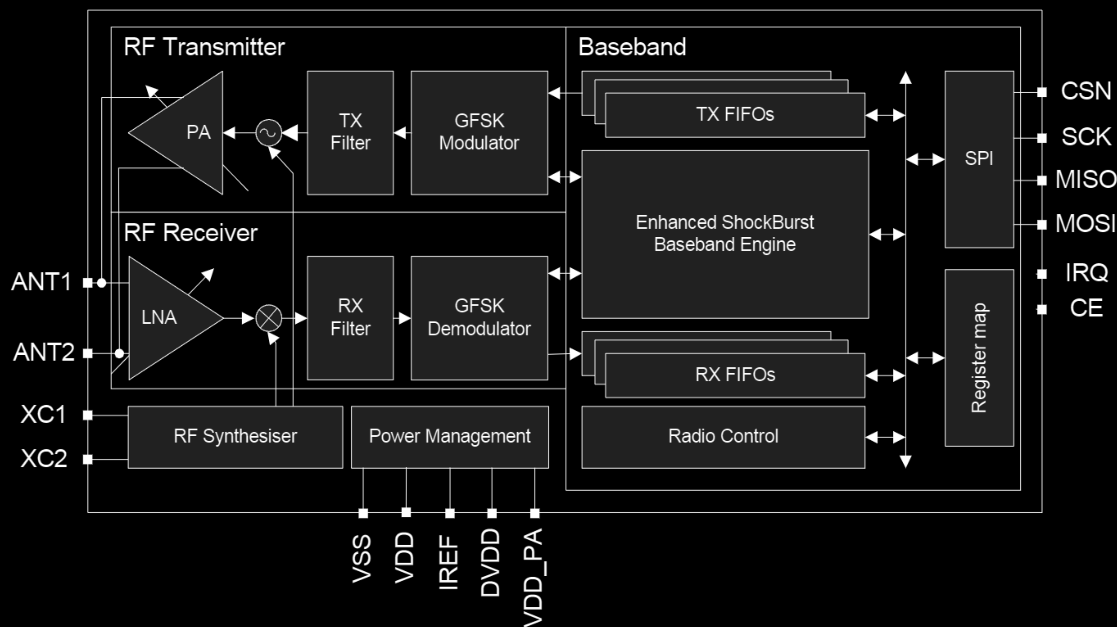
Figure 1. nRF24L01+ block diagram
