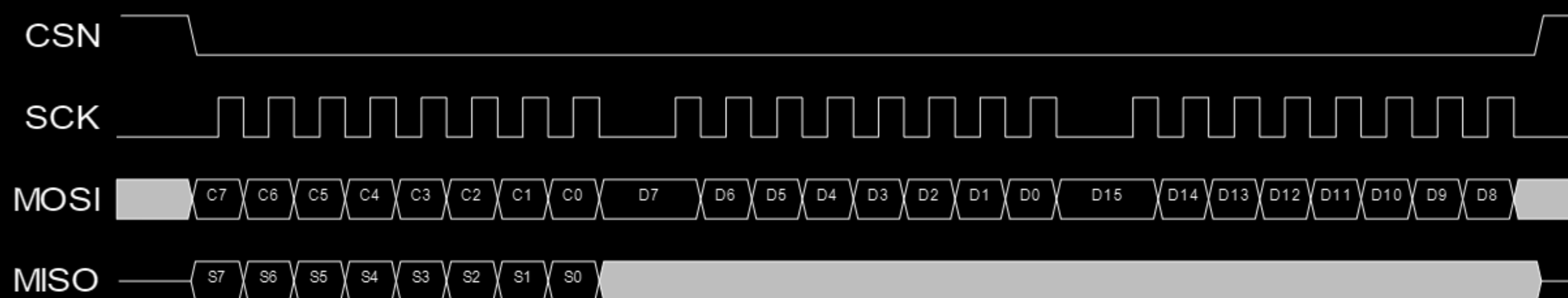
Figure 27. SPI write operation
