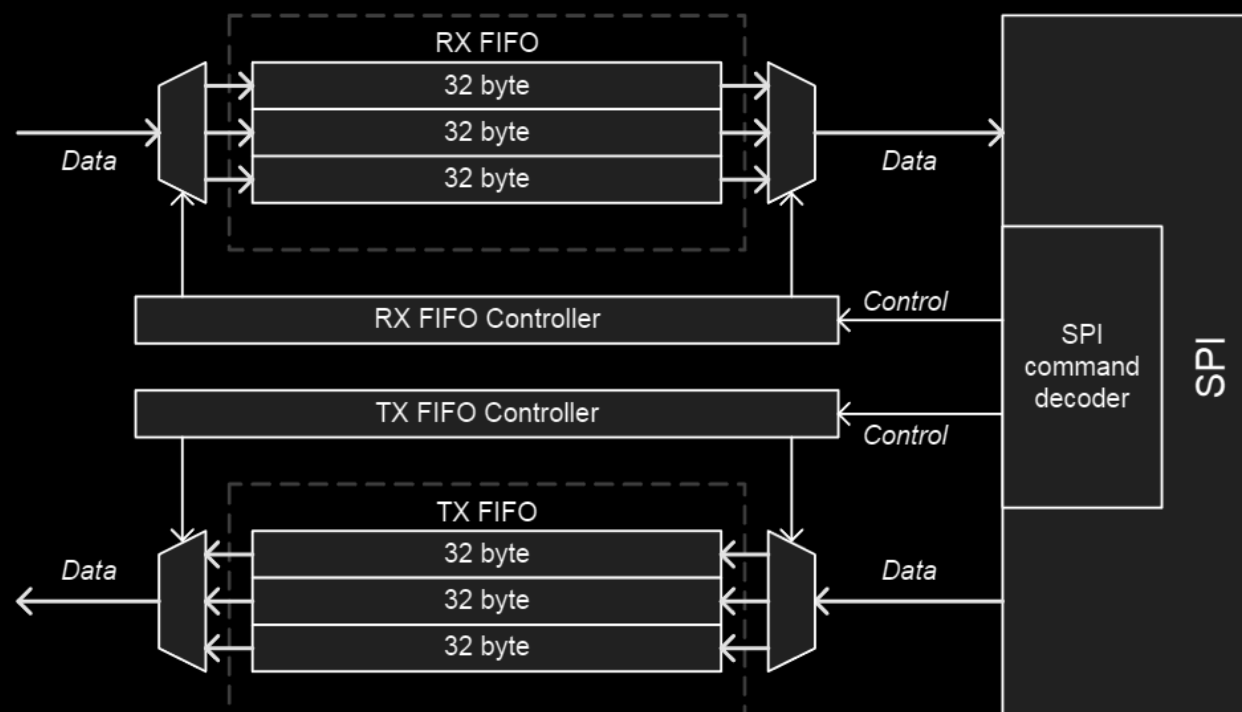
Figure 30. FIFO (RX and TX) block diagram
