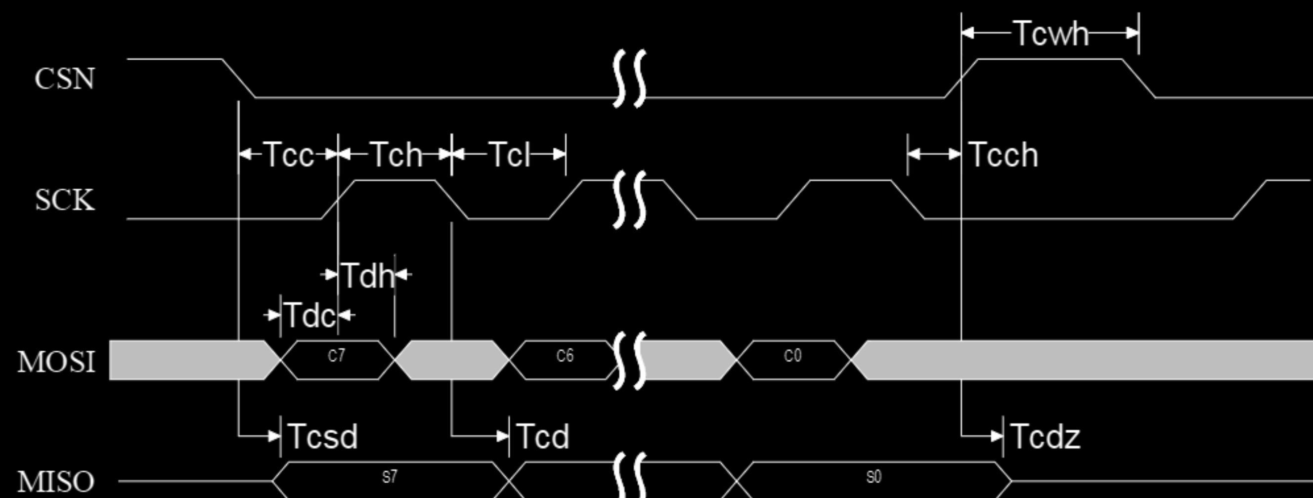
Figure 28. SPI NOP timing diagram
