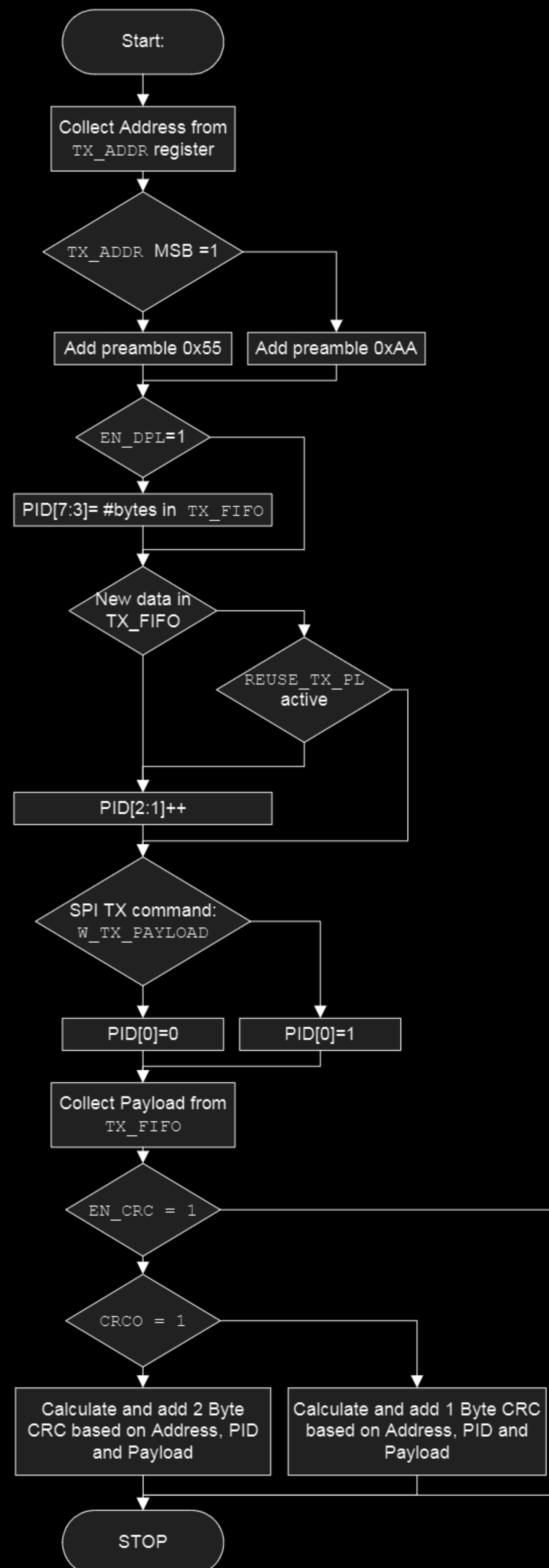
Figure 7. Automatic packet assembly
