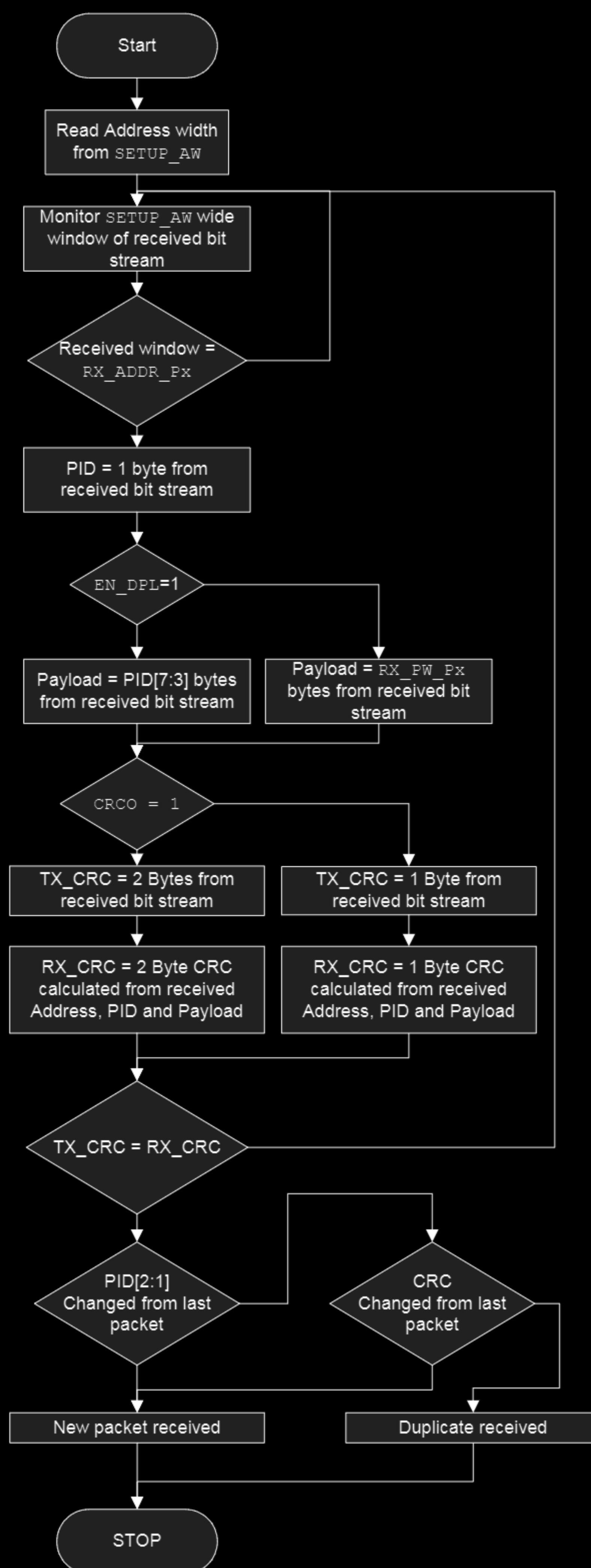
Figure 8. Automatic packet disassembly
