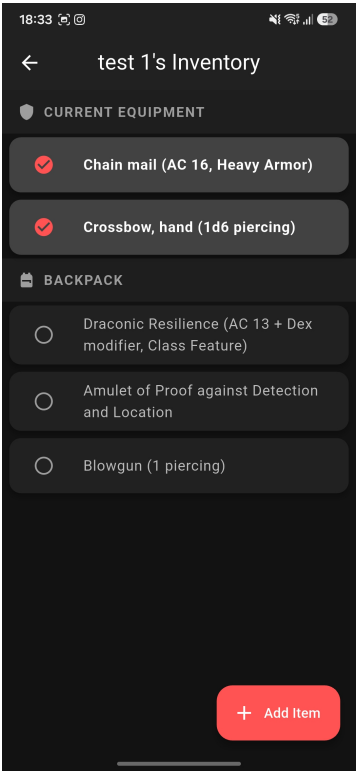
Figure 10: Inventory Screen
