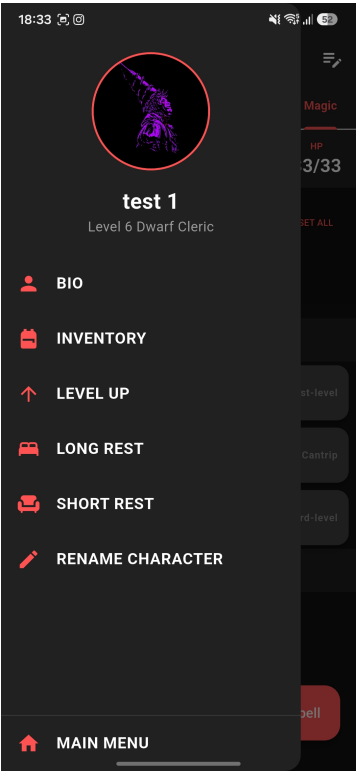
Figure 9: Navigation Drawer
