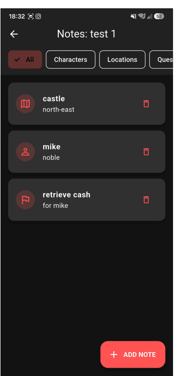
Figure 8: Notes Screen
