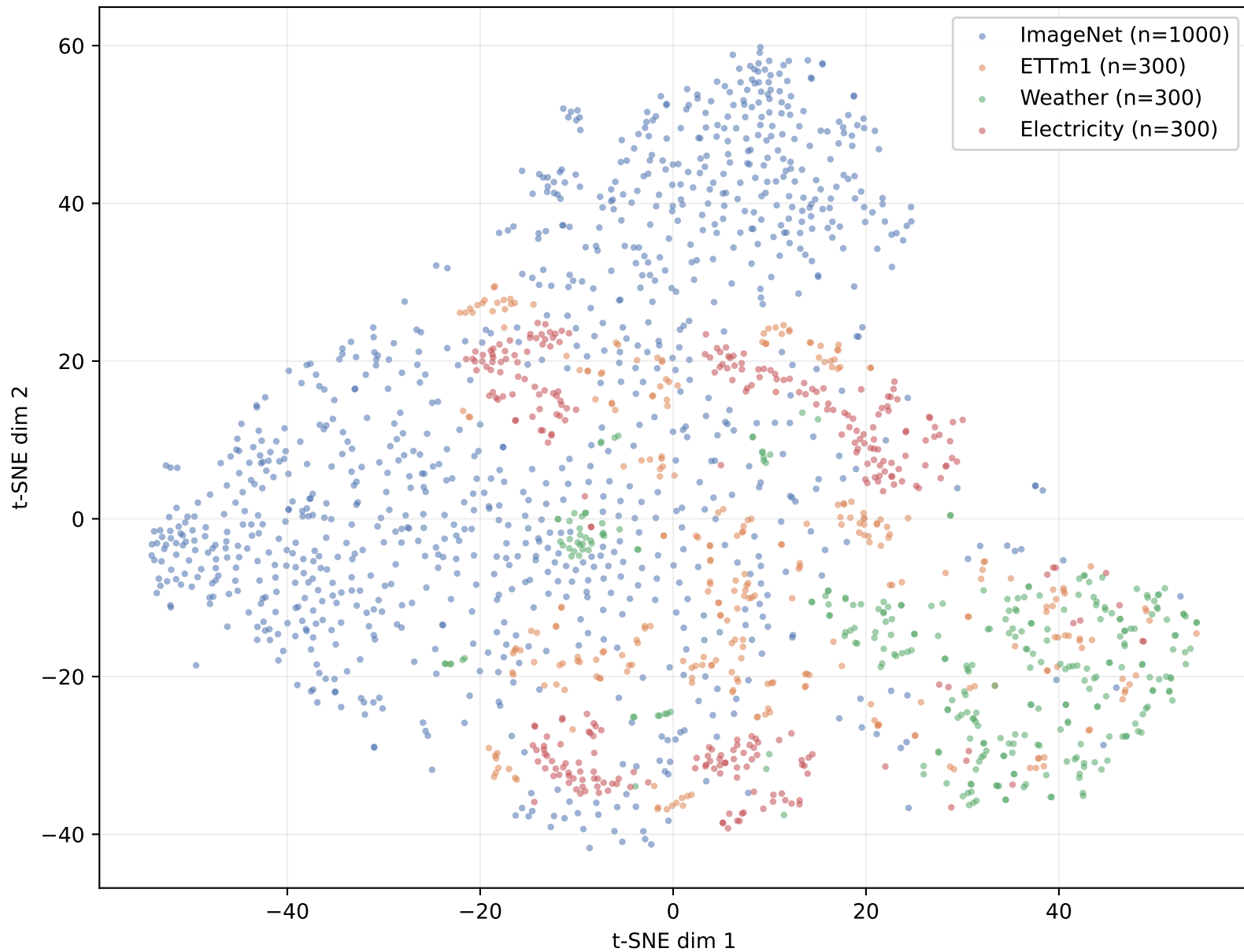
VisionTS Fig. 7 partial reproduction MAE encoder features, ImageNet + ETTm1 + Weather + Electricity (joint t-SNE)
