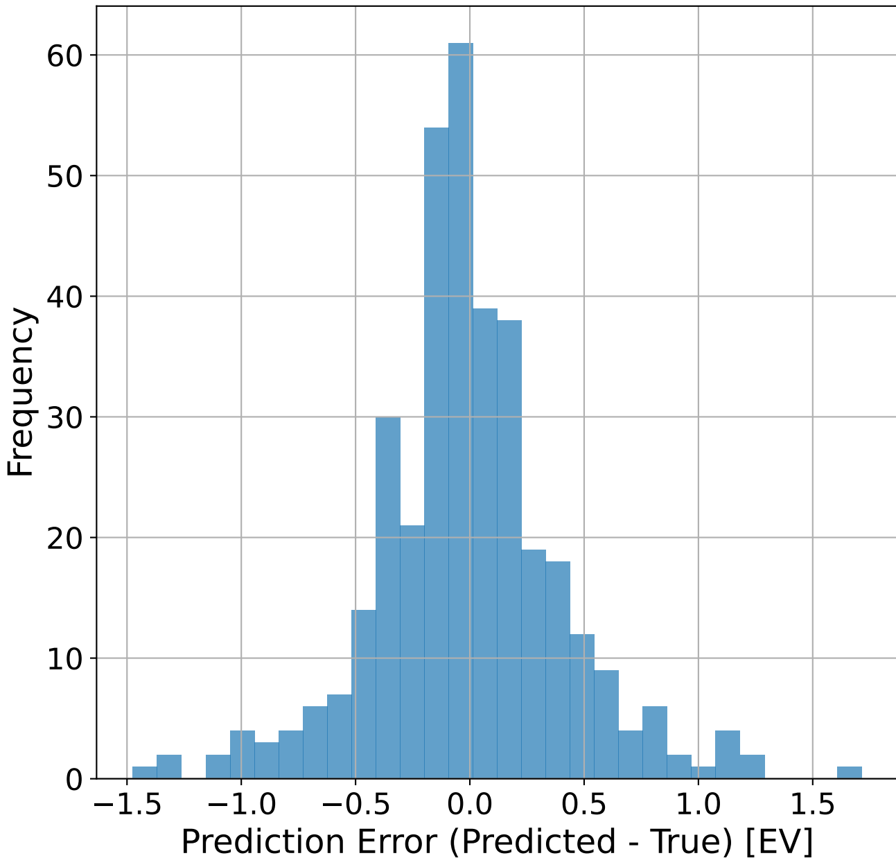
Prediction Error Distribution (RMSE=0.416)
