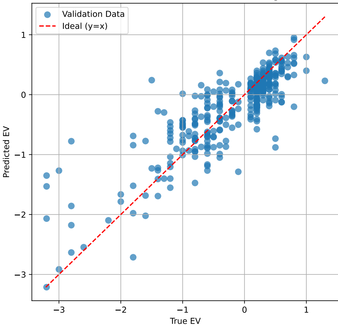
Predicted vs. True EV Scatter Plot (Training/Val)
