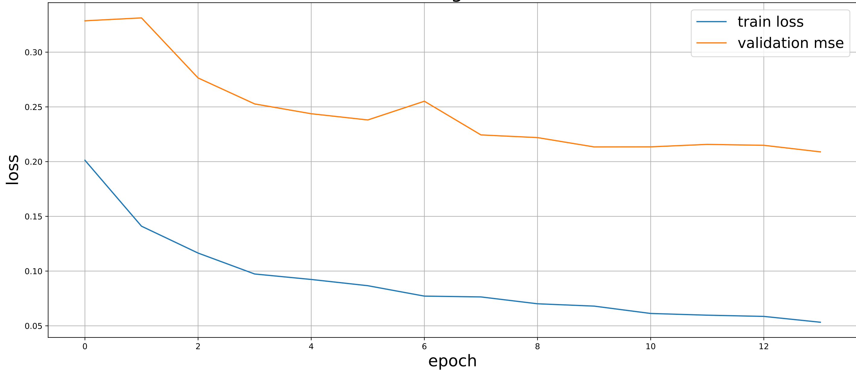
Learning Curve
