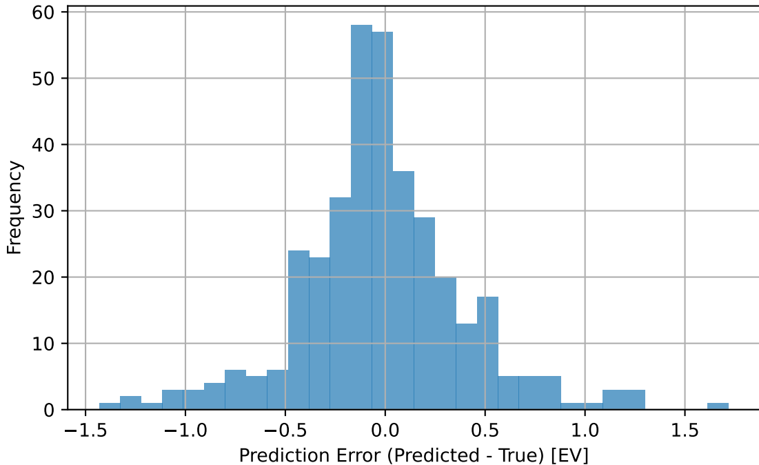
Prediction Error Distribution (RMSE=0.416)
