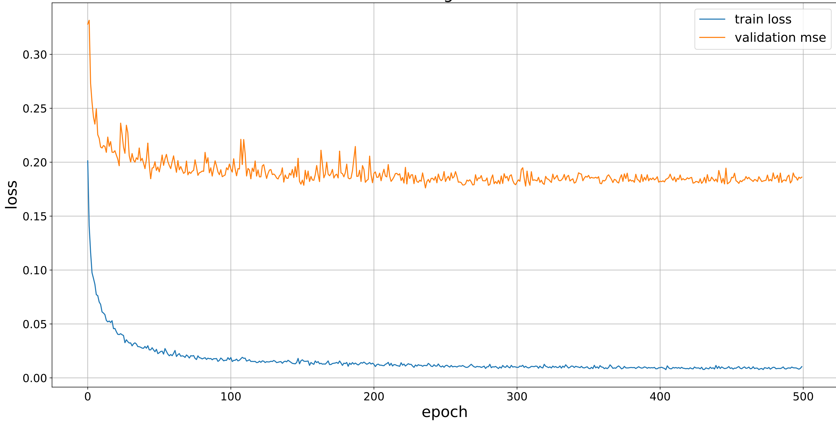
Learning Curve
