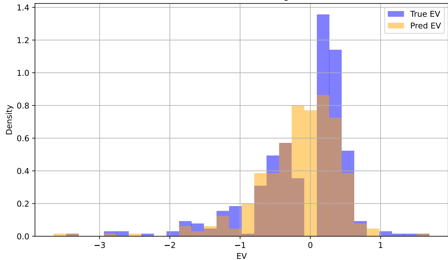
True vs Pred Distribution (KL Divergence = 0.6916)
