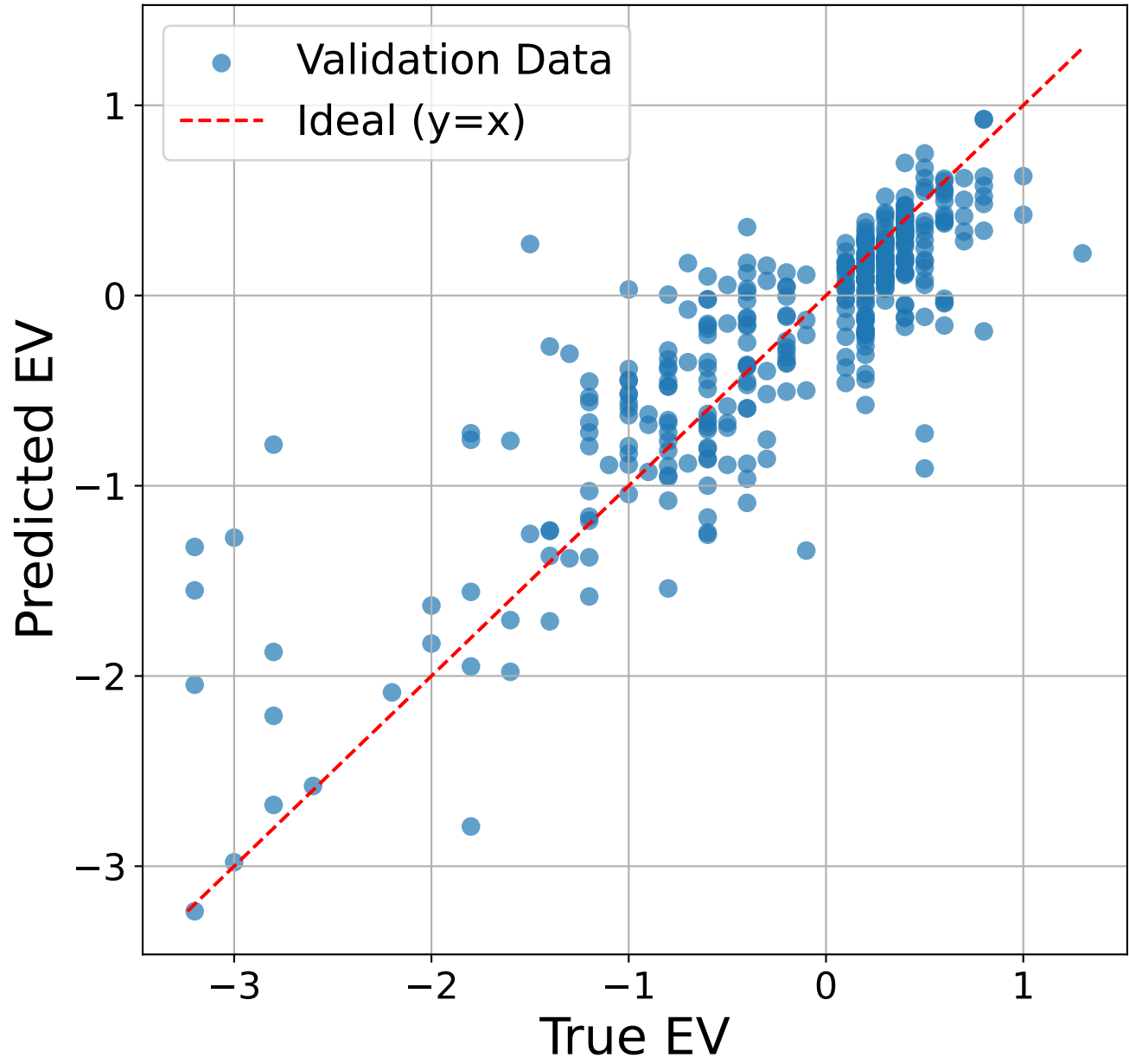
Predicted vs. True EV Scatter Plot (Training/Val)
