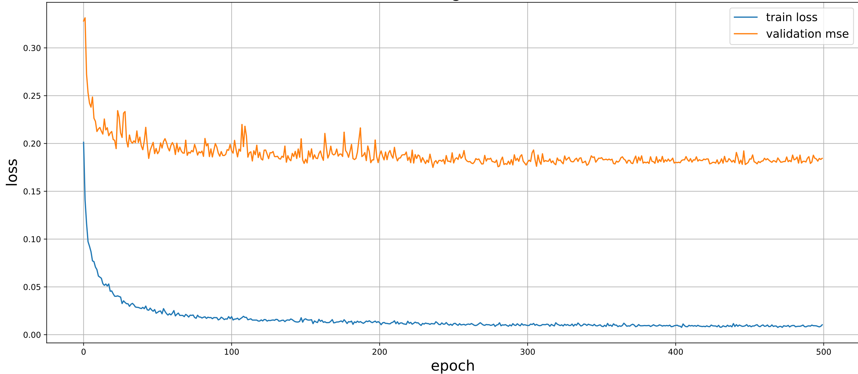
Learning Curve
