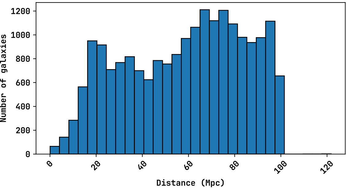
Clean GWGC - Distance (Mpc)
