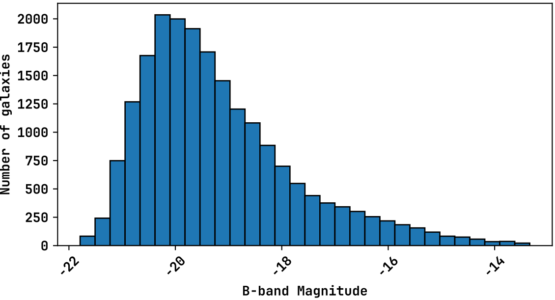
Clean GWGC - B-band Magnitude
