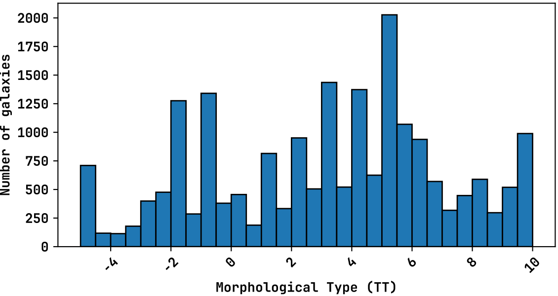
Clean GWGC - Morphological Type (TT)
