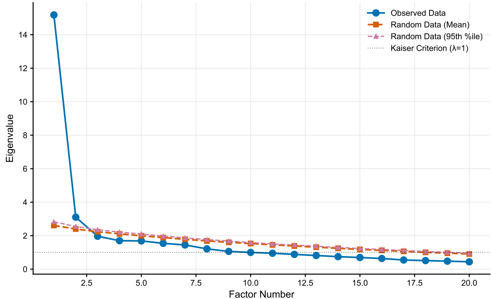
Parallel Analysis: Scree Plot
