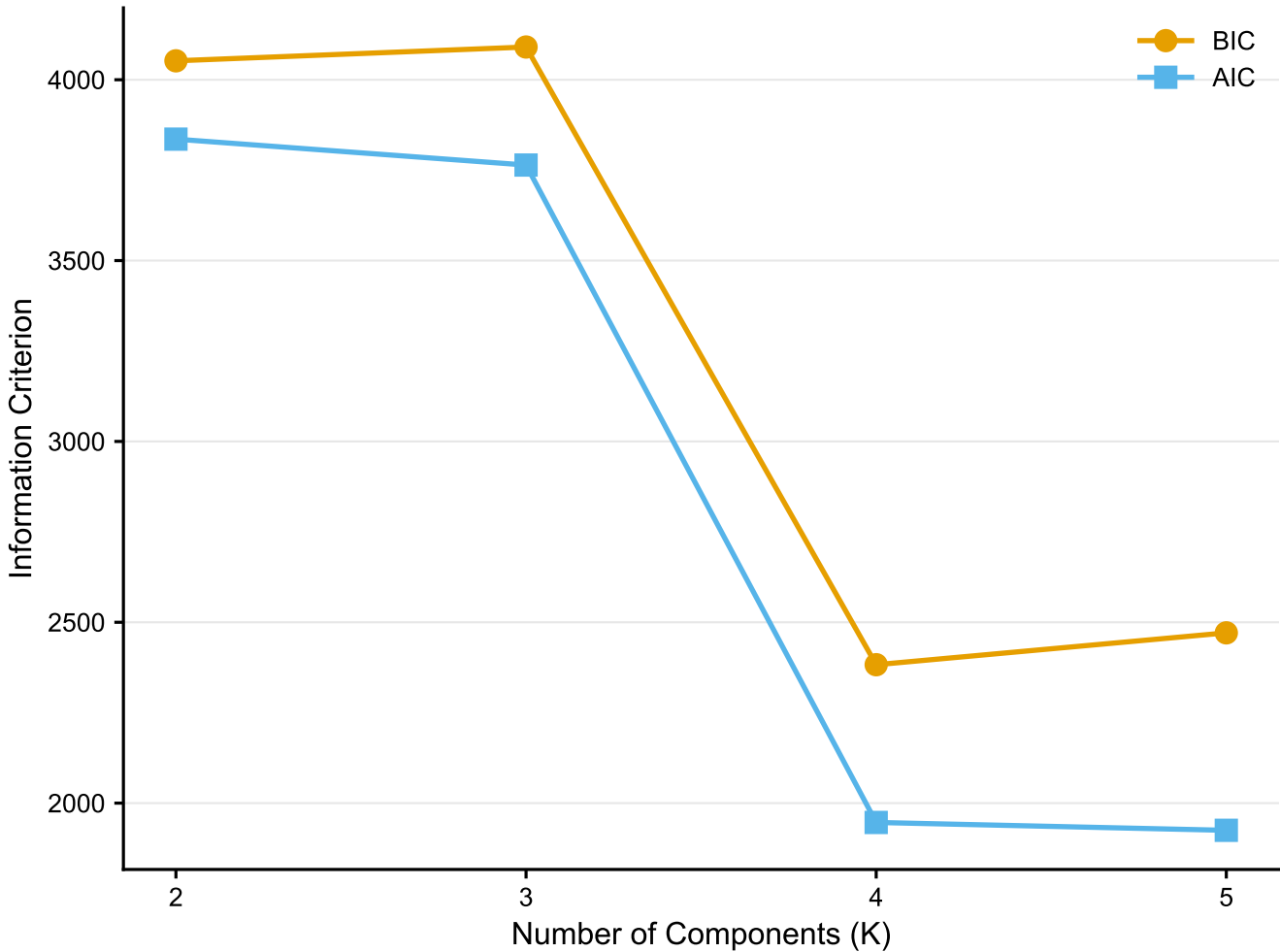
Mixture Model Selection
