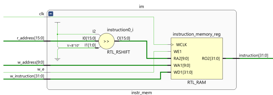
Figure 17: RTL model of instruction mem.
