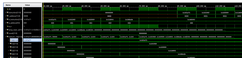
Figure 18: Waveform view of the instruction memory being loaded by instructions specified by w_instruction at address w_address .
