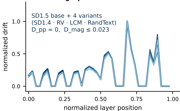
(A) Same architecture, different weights → same fingerprint
