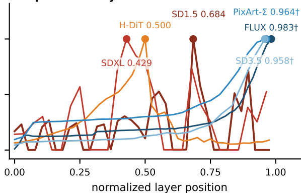
(B) Different architectures → two morphologies, not predicted by textbook labels
