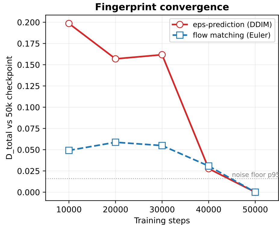
Fig. 3: DiT-S/2 Training Crystallization — eps vs flow matching
