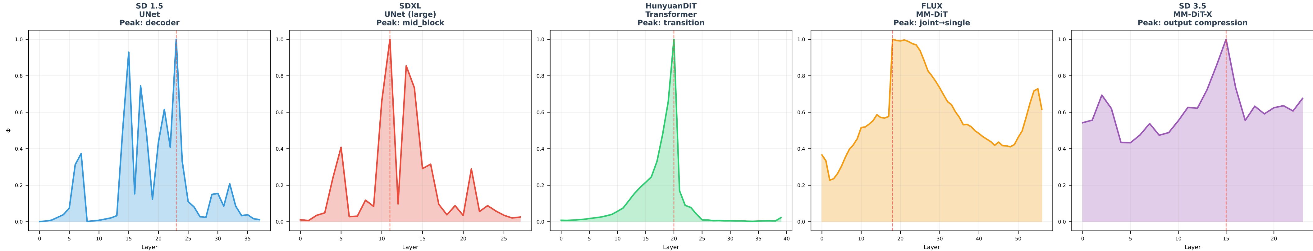
Figure 3: Topology → Fingerprint — Drift Peaks at Architecture-specific Bottlenecks
