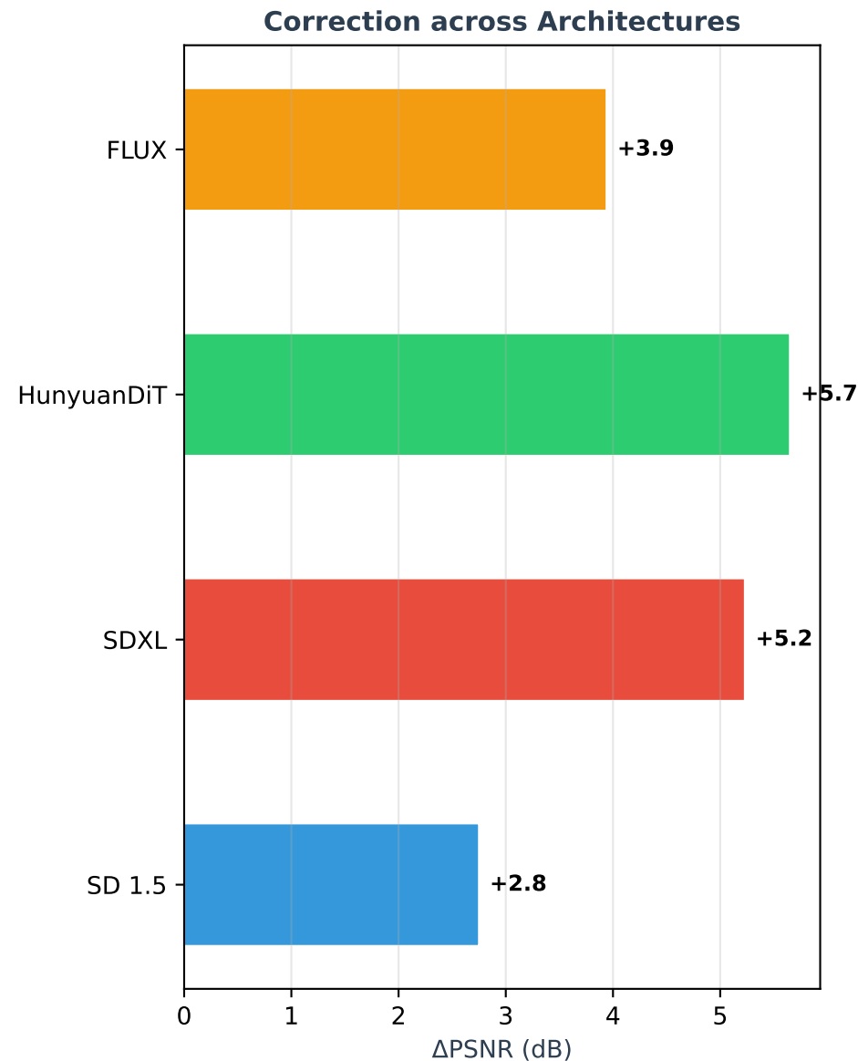
Figure 5: Diagnosis-guided Correction — Simple because Diagnosis is Sufficient
