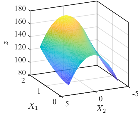
Expected-CVaR policy with QDR
