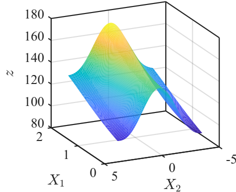
Expected-CVaR policy within RKHS
