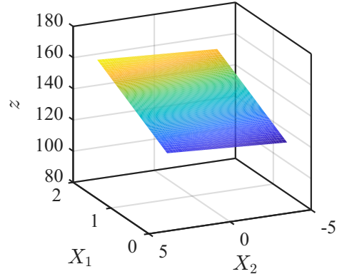
Expected-CVaR policy with LDR
