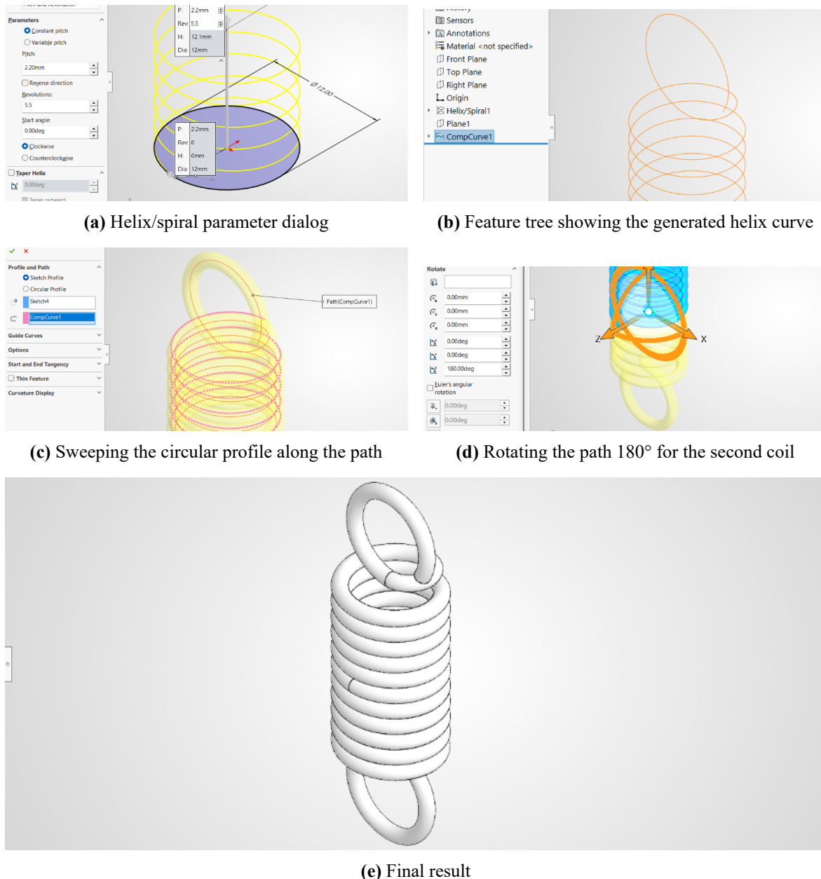
Figure 2.6: Snapshots while Designing Object 6 in Solidworks
