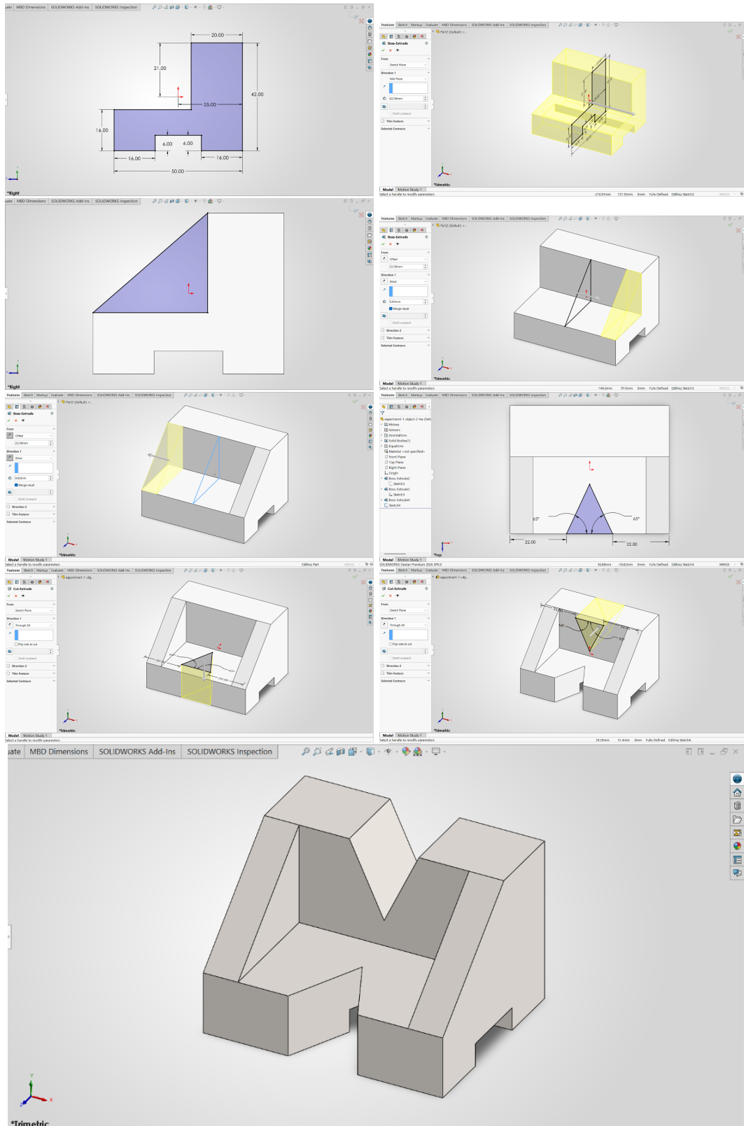
Figure 1.2: Snapshots while Designing Object 2 in Solidworks
