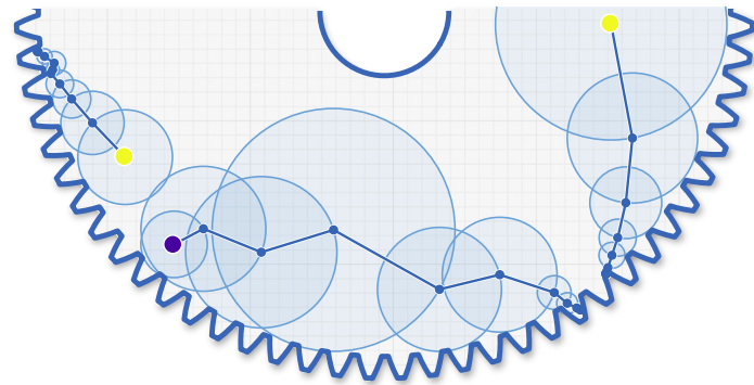
Reference
