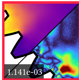
HC (3.26s)
