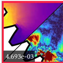
MVC (4.18s)
