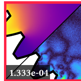
Ours (3.01s)
