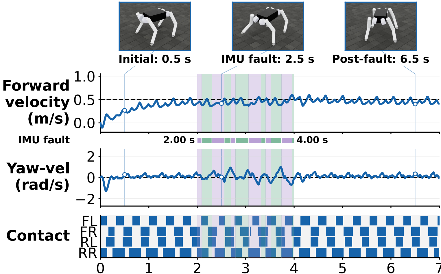
— LocoDyad — MLP-E2E (Aux) ---- Command (a) LocoDyad
