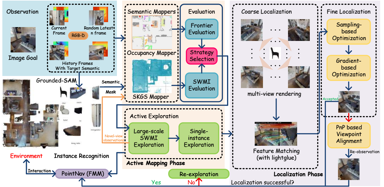
Fig. 2: Our framework comprises four modules: Mapping, Exploration, Localization, and Re-exploration. During the mapping–exploration phase, Gaussian optimization guided by target-category keyframes and SWMI-based pose selection form a closed loop, refining past observations and guiding future ones to improve target-category Gaussians and their neighborhoods. Coarse localization finds correspondences via multi-view rendering and feature matching. Fine localization estimates the goal-image capture pose using sampling- and gradient-based optimization, supplemented by PnP-based viewpoint alignment when additional verification is needed. If exploration stalls without goal confirmation, Re-exploration revisits rejected candidates for supplementary observations.
