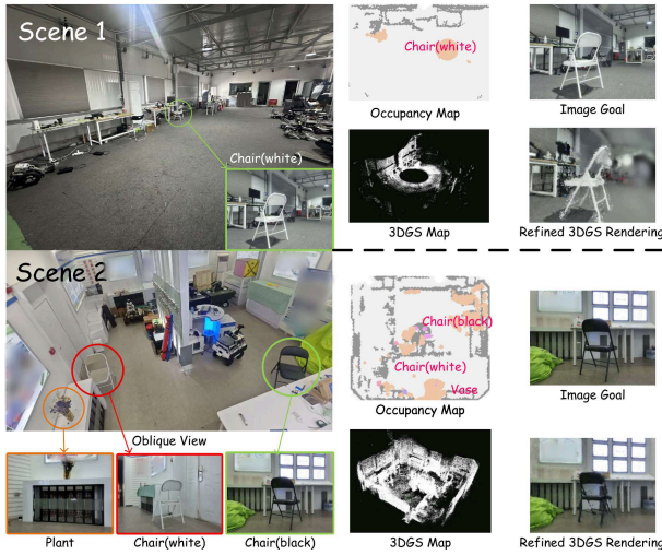
Fig. 6: Selected visualization results of the real-world experiments.
