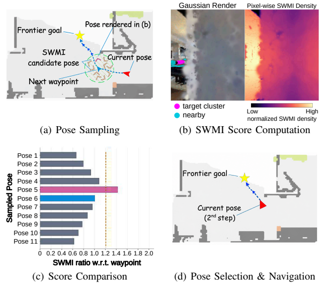
Fig. 3: One step of SWMI-guided exploration. (a) Candidate sampling: N_{\text{pose}} poses are sampled within radius r of the next FMM waypoint \sigma_t^W , which is also included in \mathcal{C}_t ; the highlighted candidate is labeled “Pose rendered in (b)”. (b) SWMI evaluation: all N_{\text{pose}} + 1 candidates are scored using 3DGS renderings and visible per-Gaussian uncertainty scores, as defined in the main text. (c) Score comparison: the example pose (pink) happens to score highest, exceeding the next waypoint (blue) and the high-information threshold \tau_h (dashed). (d) Goal selection: the example pose is selected by the double-threshold rule in Eq. (10).
