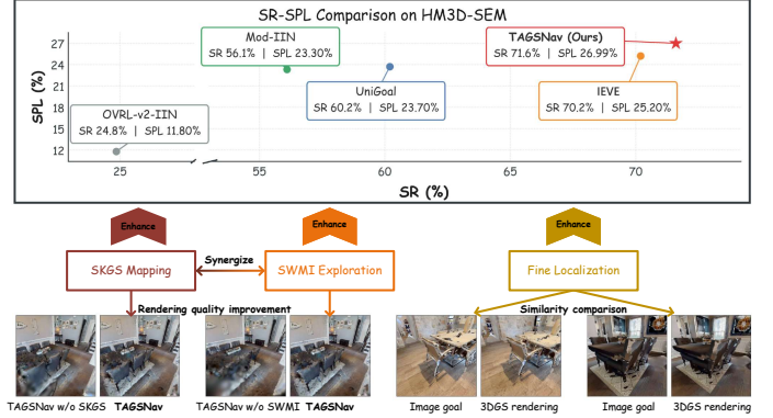
Fig. 1: SKGS mapping and SWMI-guided exploration work synergistically to improve the reconstruction quality of target-category Gaussians and their neighborhoods. Fine localization performs pose refinement and matching to estimate the goal-image capture pose. Together, these components improve SR and SPL in IIN.
