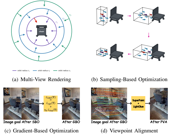
Fig. 4: Coarse-to-fine localization with conditional PVA: The first two panels illustrate viewpoint sampling and selection, whereas the latter two visualize the subsequent localization procedures based on the selected rendered viewpoint.
