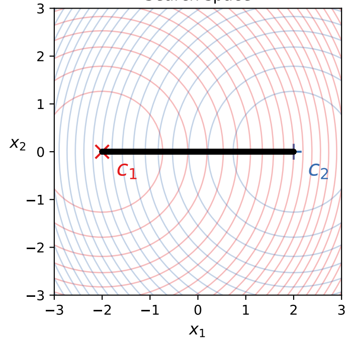
Search space
