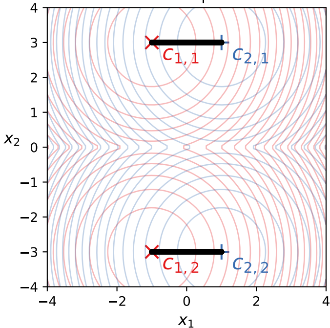
Search space
