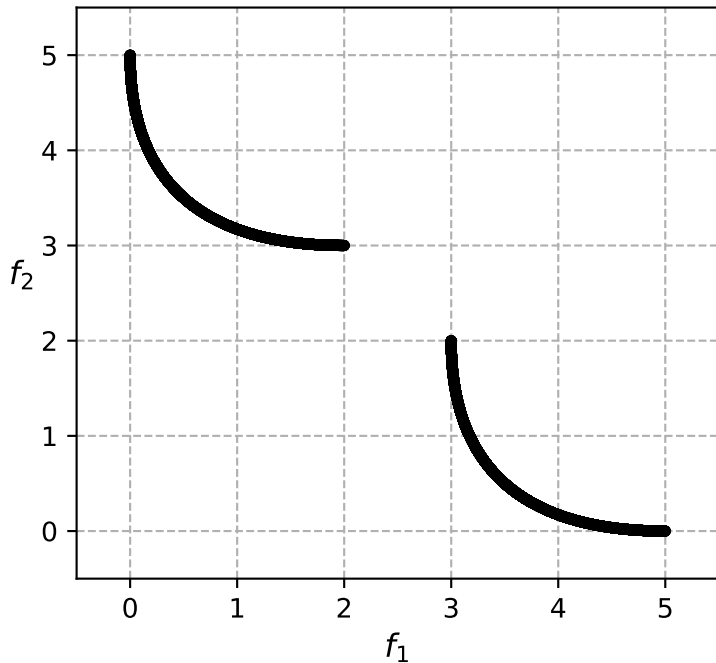
Disconnected convex Pareto front
