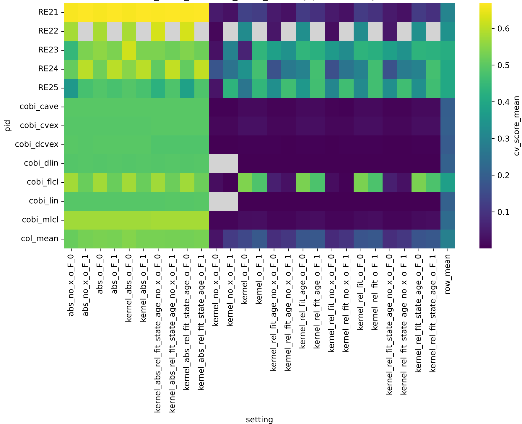
cv_score_mean: cv_score_mean by pid vs setting
