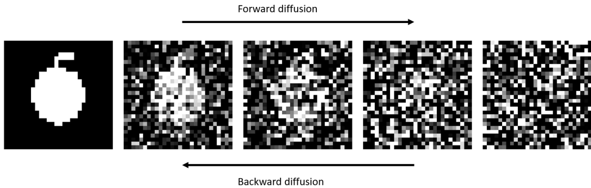
Figure 3: First we created an image of an apple, and added noise step by step (forward diffusion). The reverse process is called backward diffusion.
