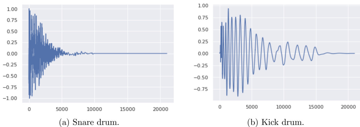
Figure 1: Examples of audio waveforms of sound. The y-axis shows the amplitude, the x-axis shows the time. Source: Rouard, Hadjeres 2021 https://crash-diffusion.github.io/crash/
