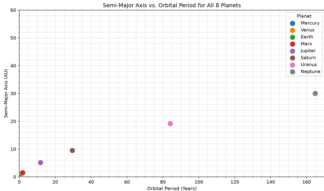
Figure 5: Period and semi major axis of all eight planets in our solar system.
