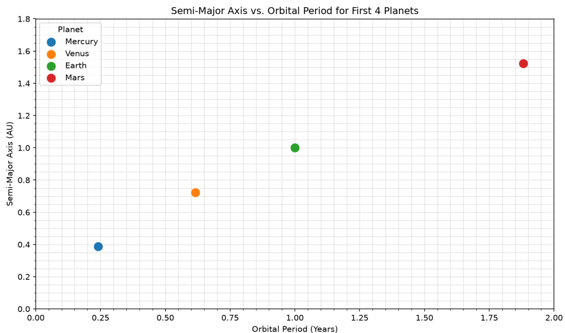
Figure 3: Orbital period and semi-major axis of the four inner planets in the Solar System.
