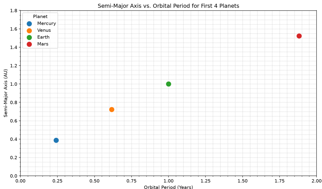
Figure 4: Period and semi major axis of the first four planets in our solar system.
