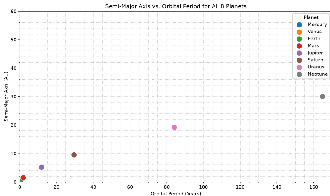
Figure 5: Period and semi major axis of all eight planets in our solar system.
