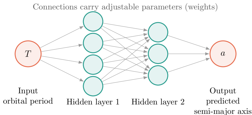
Figure 6: A simplified neural network that uses the orbital period T to predict the semi-major axis a . During training, the network adjusts the parameters of the connections to reduce the loss function.
