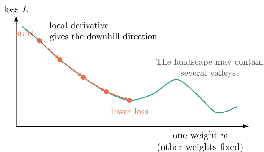
Figure 7: Gradient descent on a one-dimensional slice of a loss landscape. At each point, the local derivative determines the downhill direction. After a small step, the derivative is calculated again. A real neural network has many weights, so its loss landscape has many dimensions.
