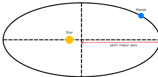
Figure 1: An elliptical planetary orbit with the semi-major axis indicated in red.
