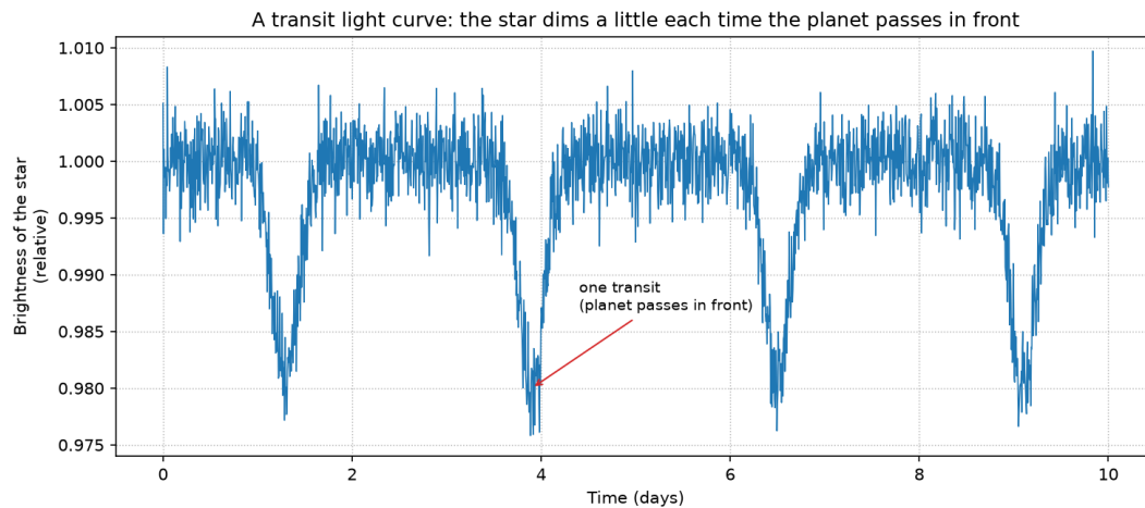
Figure 8: A transit light curve: each time the planet passes in front of its star, the measured brightness dips a little. Real data are noisy, and most dips are not caused by planets.
