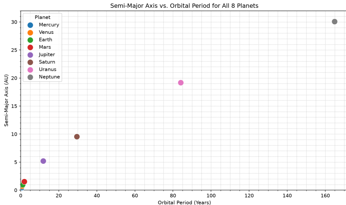
Figure 2: Orbital periods and semi-major axes of the planets in the Solar System.
