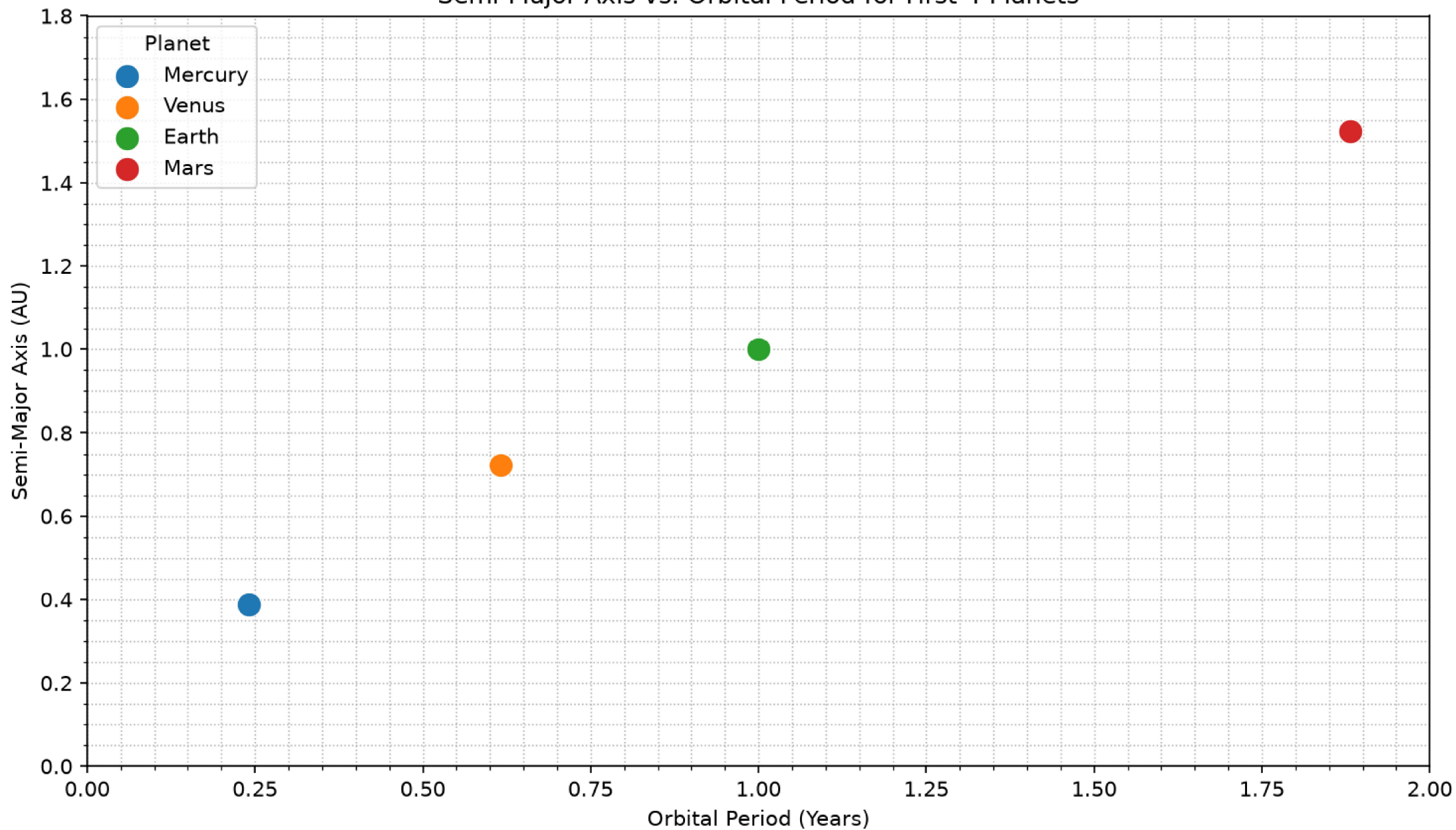
Semi-Major Axis vs. Orbital Period for First 4 Planets
