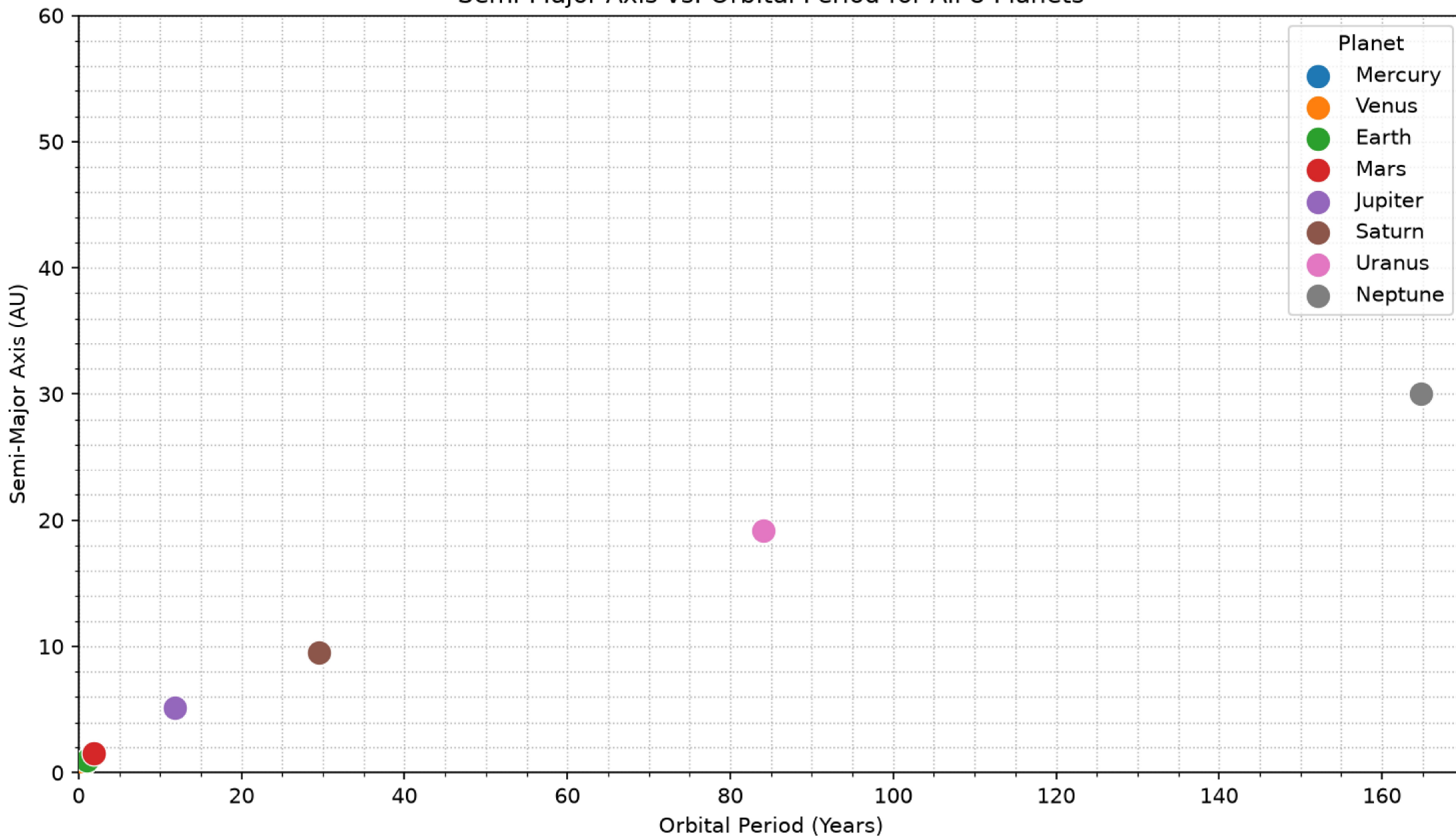
Semi-Major Axis vs. Orbital Period for All 8 Planets
