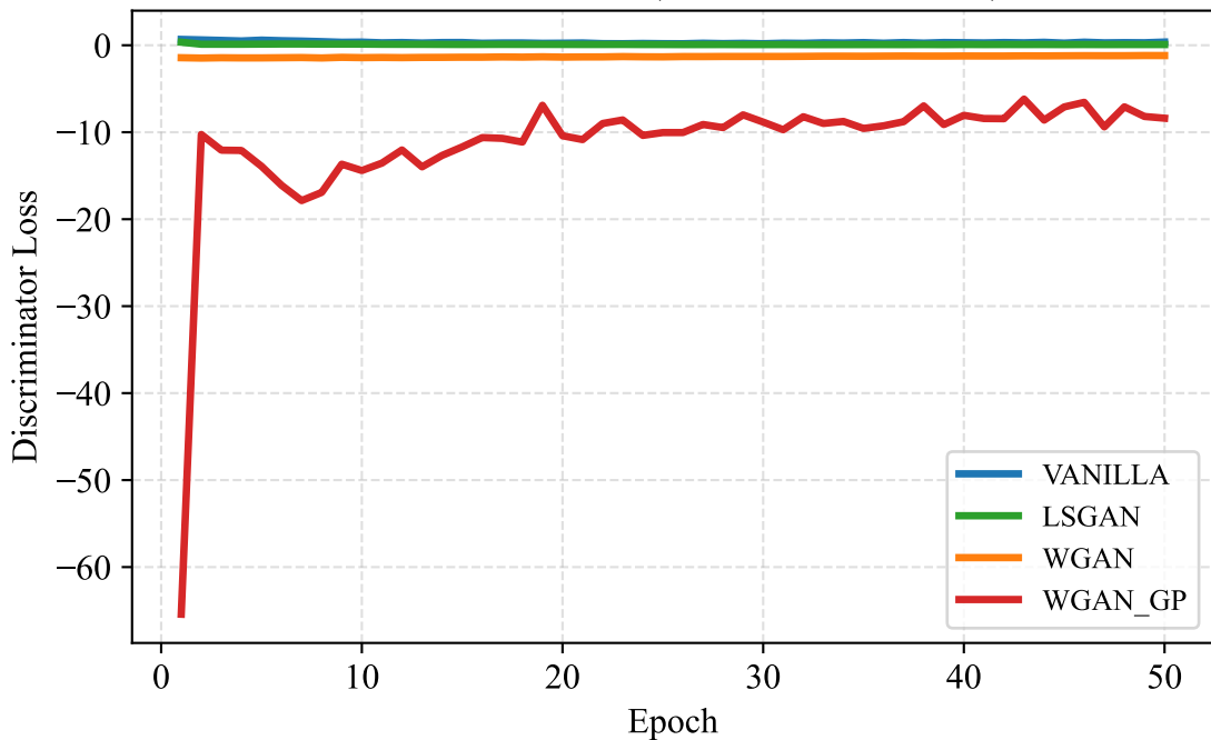
Discriminator Loss (Dataset Size = 10000)
