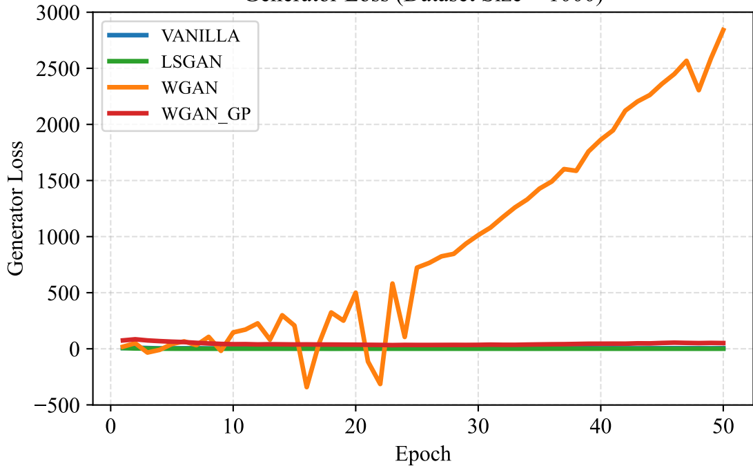
Generator Loss (Dataset Size = 1000)
