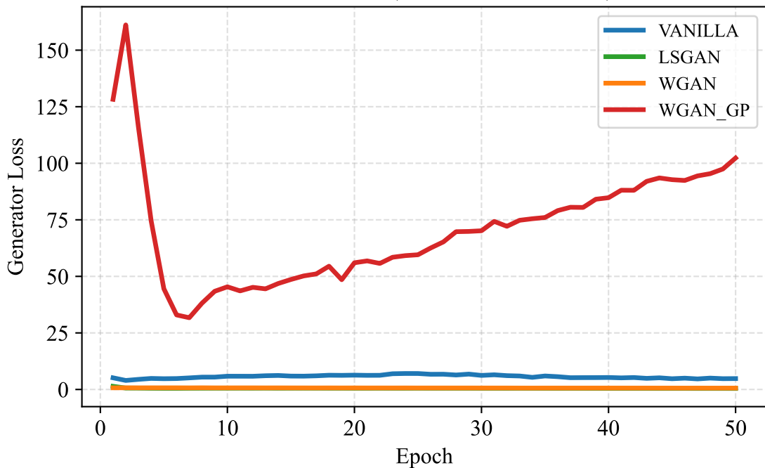
Generator Loss (Dataset Size = 10000)
