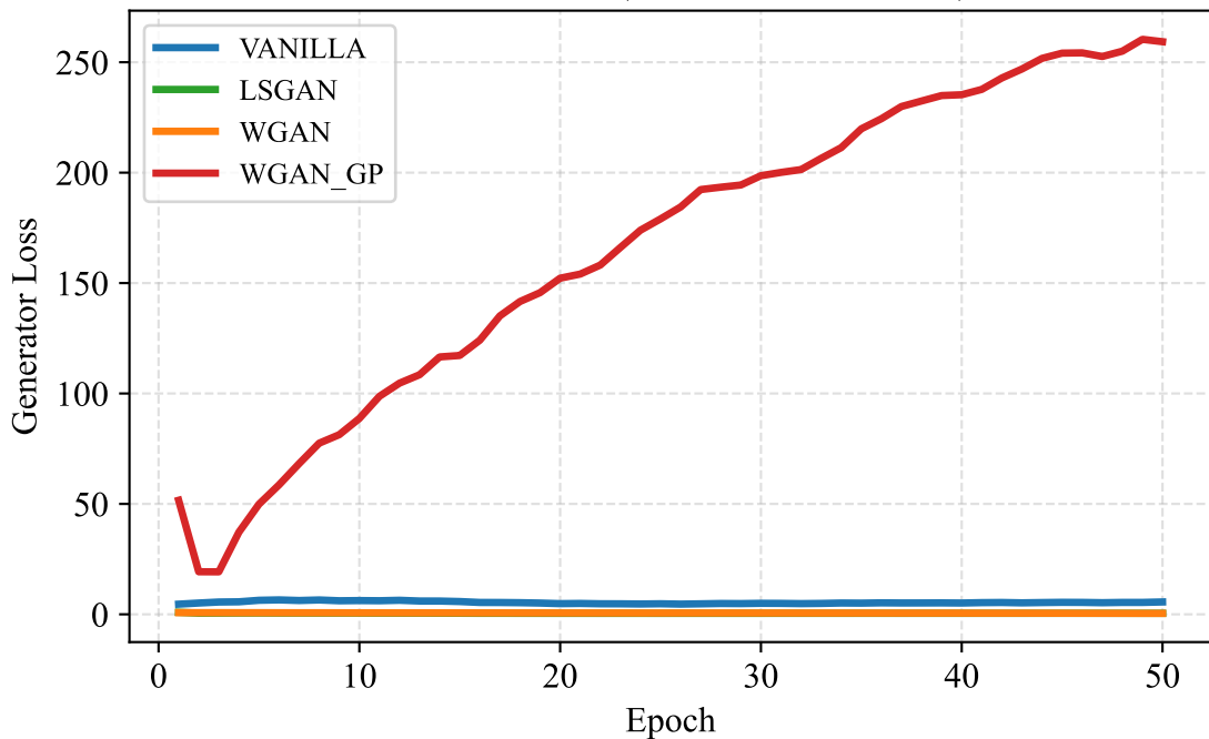
Generator Loss (Dataset Size = 25000)
