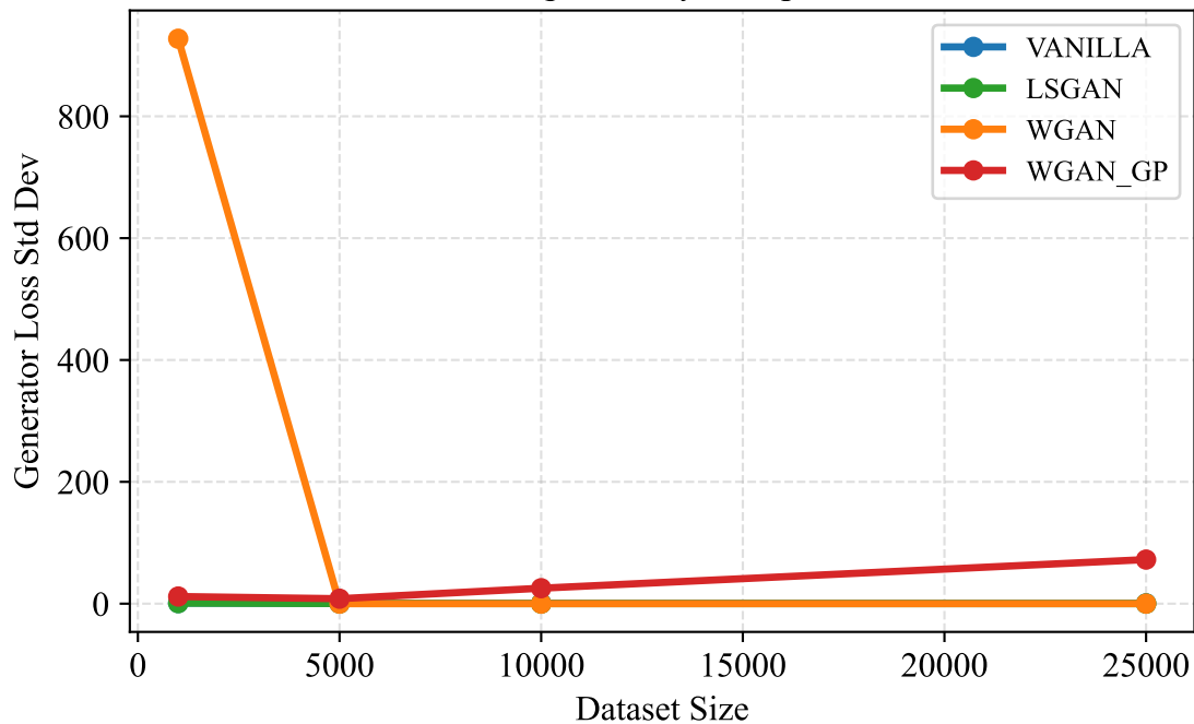
Training Stability Comparison
