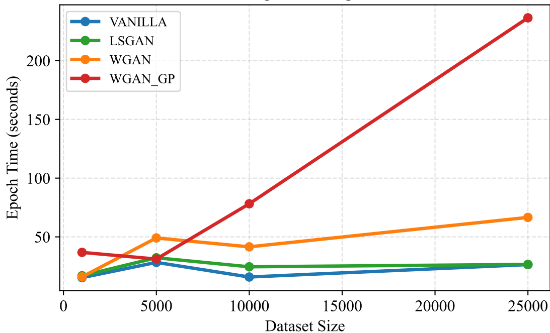
Training Cost Comparison
