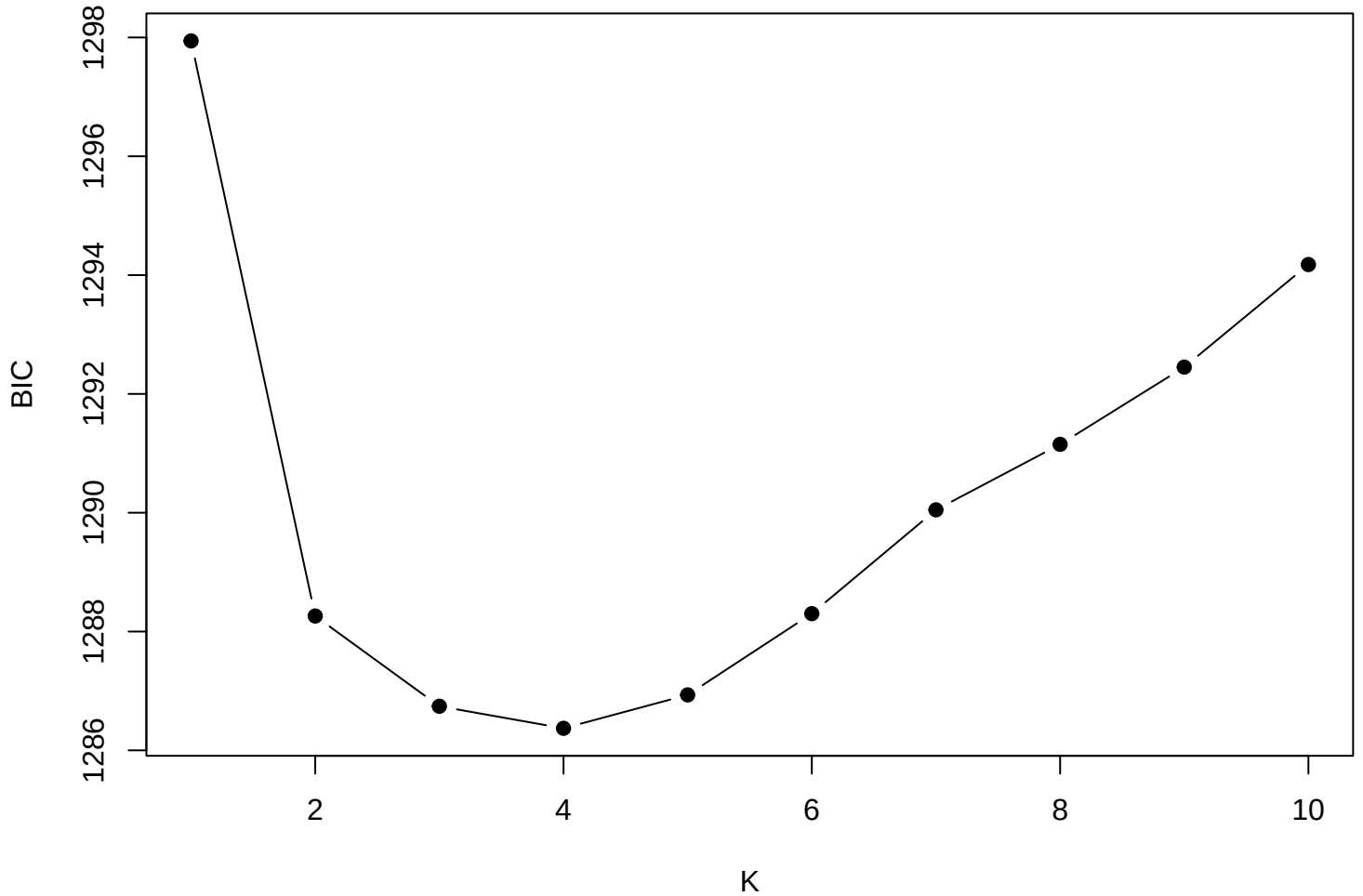
Optimal K by BIC
