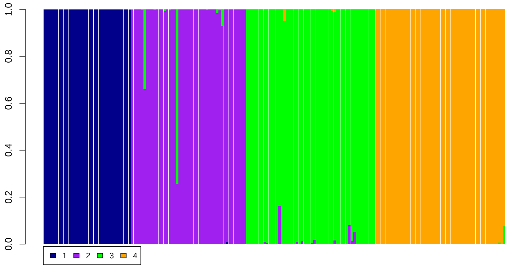
membership probability
