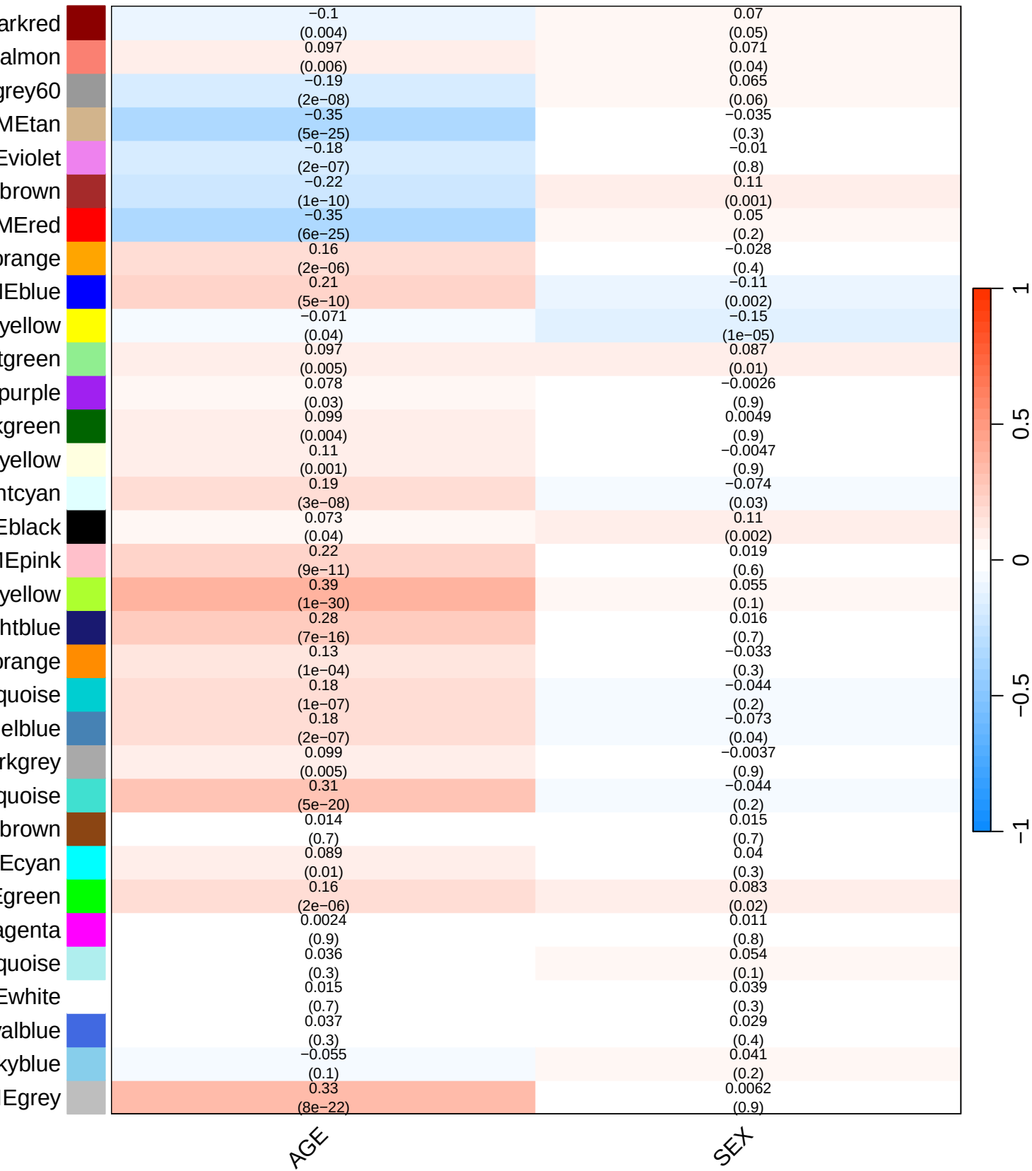
Module-trait relationships
