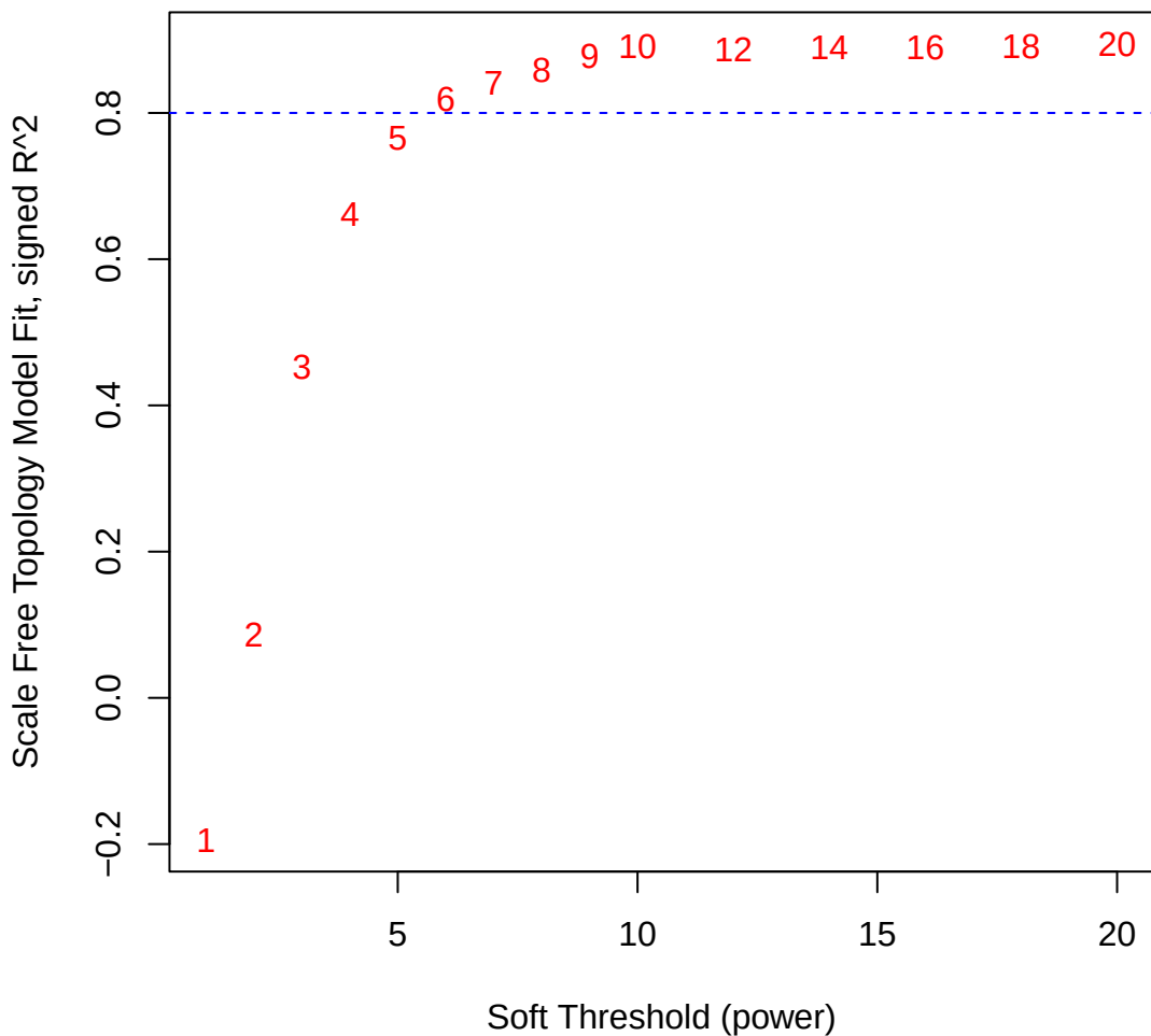
Scale independence
