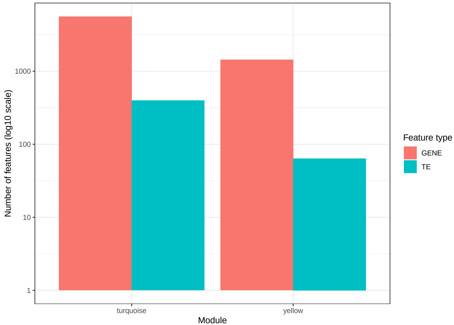
Gene and ERV composition of WGCNA1 ERV-rich modules
