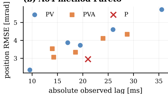
(b) A04 method Pareto
