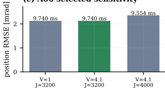
(c) A06 selected sensitivity
