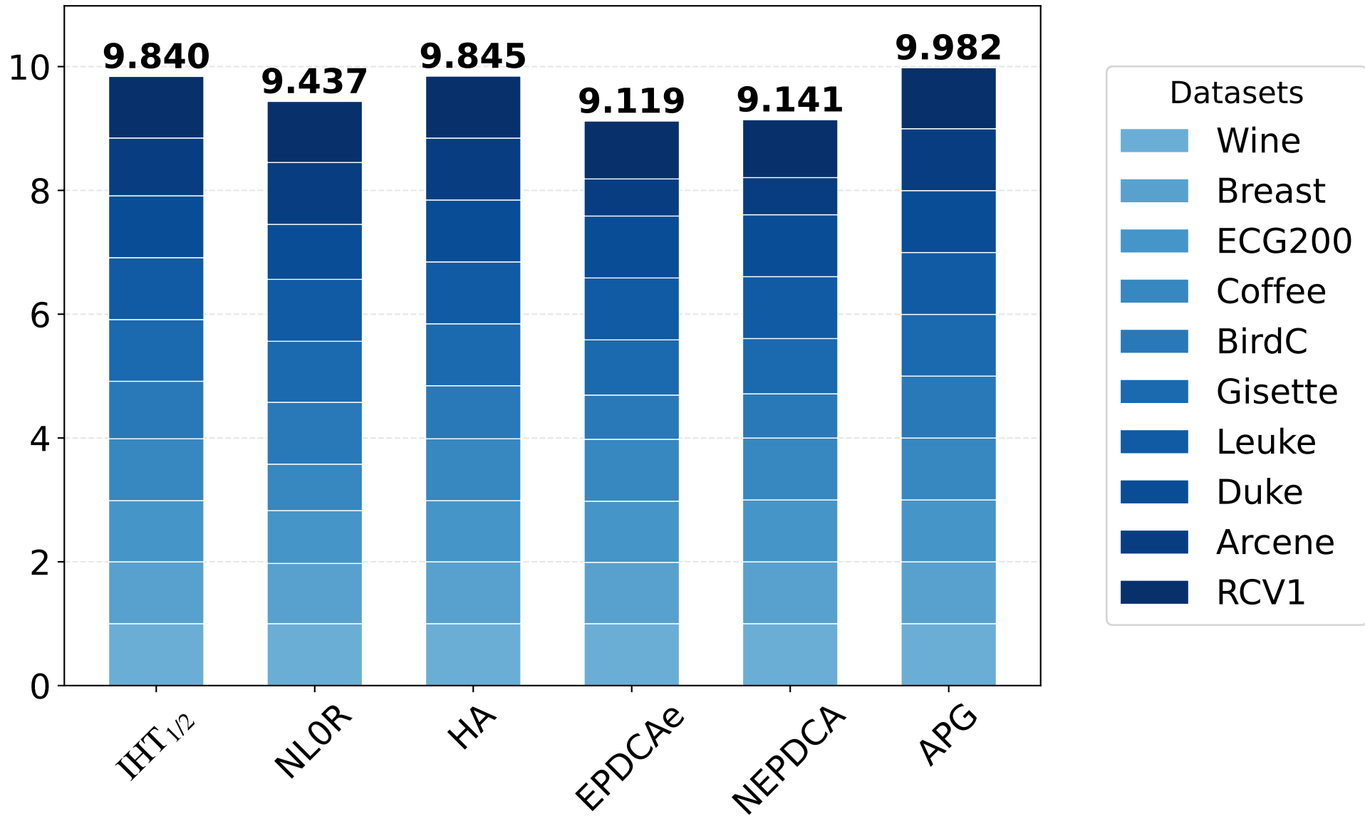
Cumulative ACCRatio
