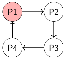
Deadlock cycle in a wait-for graph
