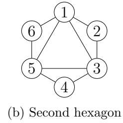
Figure 4: Two distinct triangulations of a cycle
